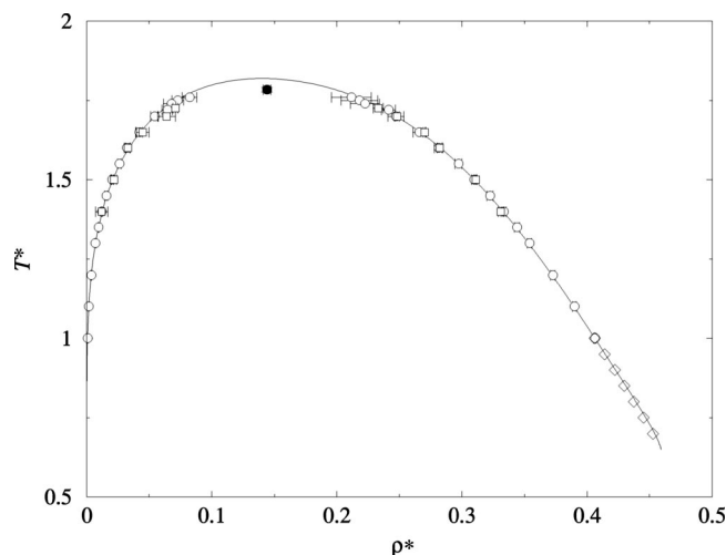
FIG. 1. Vapor-liquid coexistence curve ( T - \rho representation) for the 2CLJ model system with L^*=1 from computer simulation (symbols) and predictions from Wertheim's TPT1 (curve). The open circles correspond to the Gibbs ensemble Monte Carlo simulation results obtained in this work, the squares to the Gibbs ensemble data obtained by other authors (see Ref. 26), the diamonds to the liquid densities obtained in this work using NPT Monte Carlo simulations at zero pressure, and the closed circle to the critical point [estimated by the scaling relations given by Eqs. (5) and (6)].
