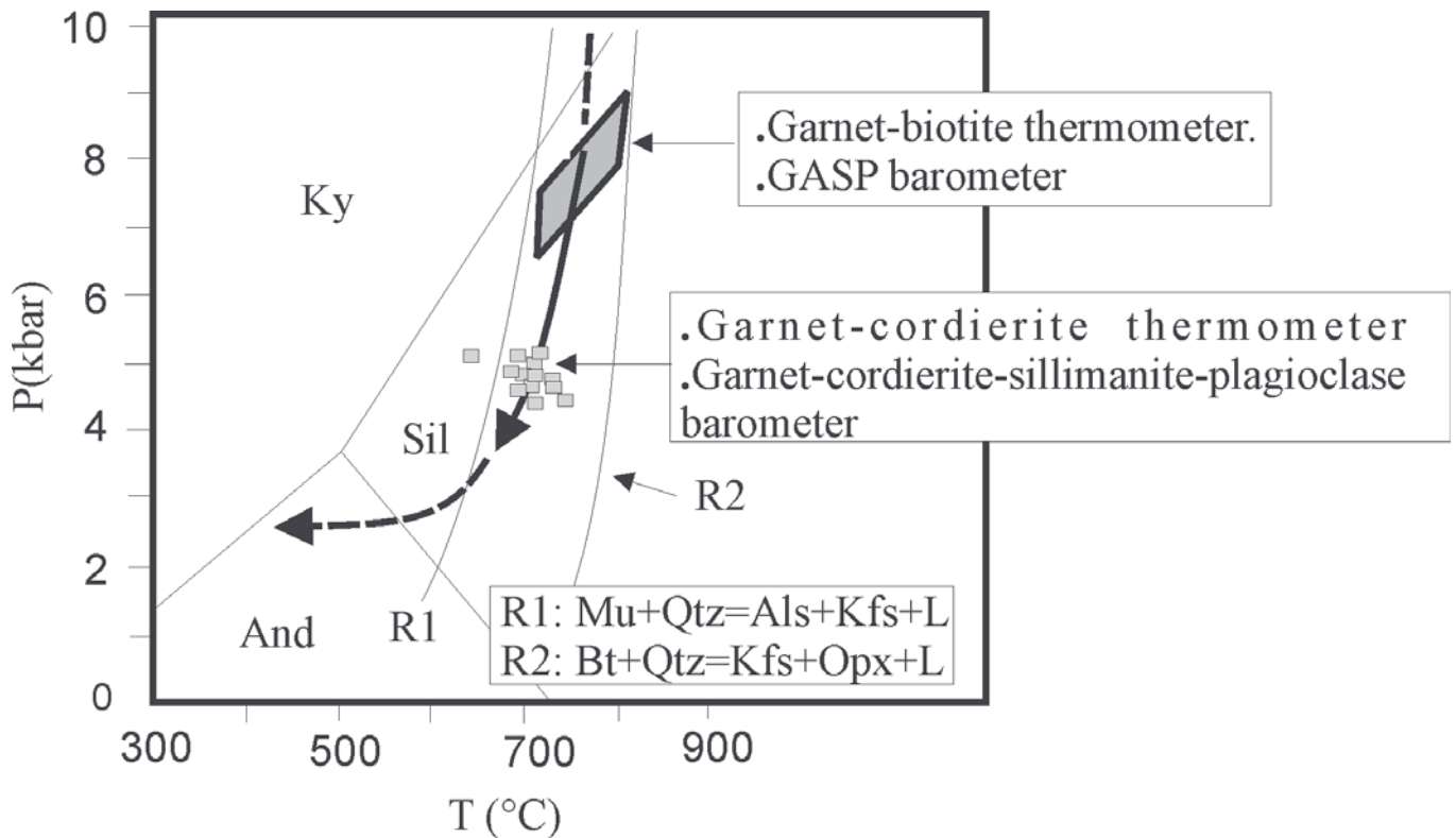
Fig. 2.- P-T diagram showing thermobarometric results and the P-T path deduced for the migmatitic paragneisses. Solid and broken lines represent segments of P-T path deduced respectively from thermobarometric estimations and textural analysis.
