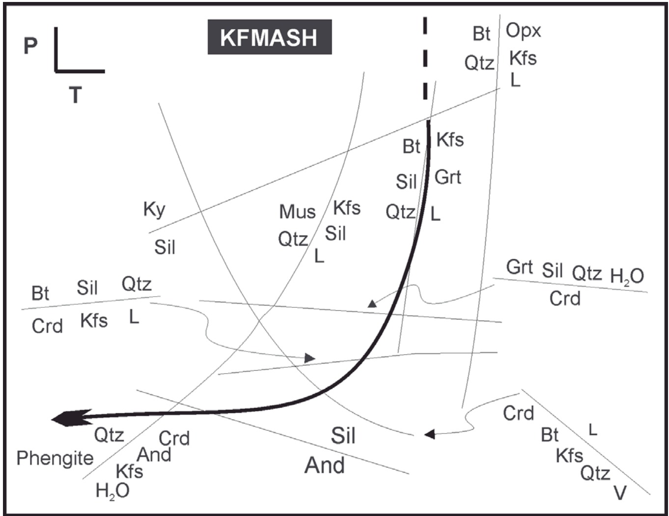
Fig. 1.- Qualitative petrogenetic grid in the KFMASH system for metapelites of intermediate bulk composition (Vielzeuf and Holloway, 1988).
