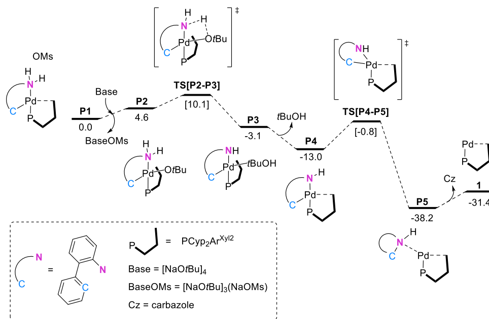
Figure 1. Gibbs energy profile for the precatalyst activation step. Energies in kcal mol -1 .
