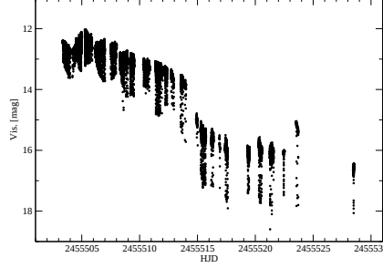
Figure 1. The photometric behavior of HT Cas in November 2010. During that time one can observe an outburst precursor, developed later on into full superoutburst. At the end of November star came back to its quiescence level.
