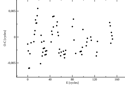
Figure 3. The O - C diagram for eclipses observed during superoutburst of HT Cas in November 2010. Regular humps are the manifestation of beat period - composition of the orbital and superhump period.
