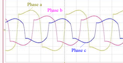
Source currents, system without compensate. 4 A/div. 5ms/div
