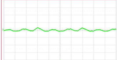
Neutral current with passive and active filter. 4 A/div. 5ms/div
