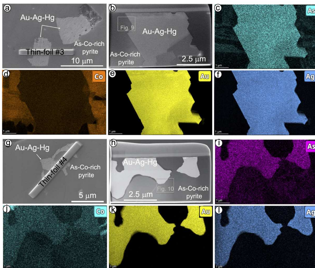
Fig. 8. A composition of back-scattered electron and negative HAADF images along with TEM-EDS elemental maps acquired for the euhedral (a-f) and anhedral (g-l) Au-Ag-Hg inclusions sampled by the thin-foil #3 and thin-foil #4 respectively from pyrite of the Tharsis deposit.
