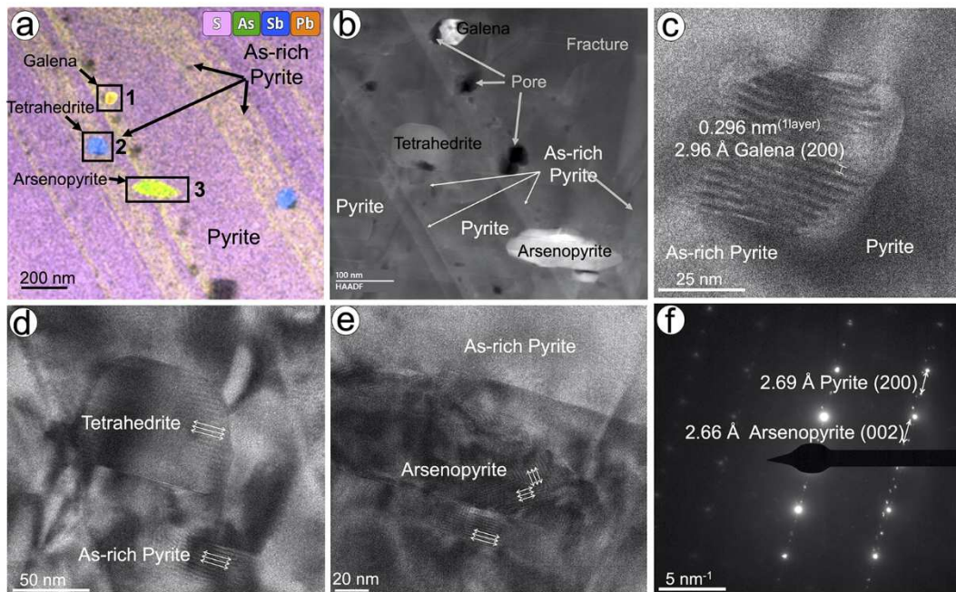
Fig. 7. Nanostructure of a selected area of the thin-foil #2 showing coexistence of nanoscale chemical zoning and metal-bearing NPs. TEM-EDS elemental and negative HAADF image of the selected area are shown in (a) and (b) respectively, whereas (c-d) are high magnification images of the NPs and their hosting pyrite matrices; (f) SAED pattern showing identical orientation of arsenopyrite NPs and host pyrite matrix. Black rectangles with numbers inset in (a) correspond to those NPs of galena (1), tetrahedrite (2) and arsenopyrite (3) shown in (c-h).
