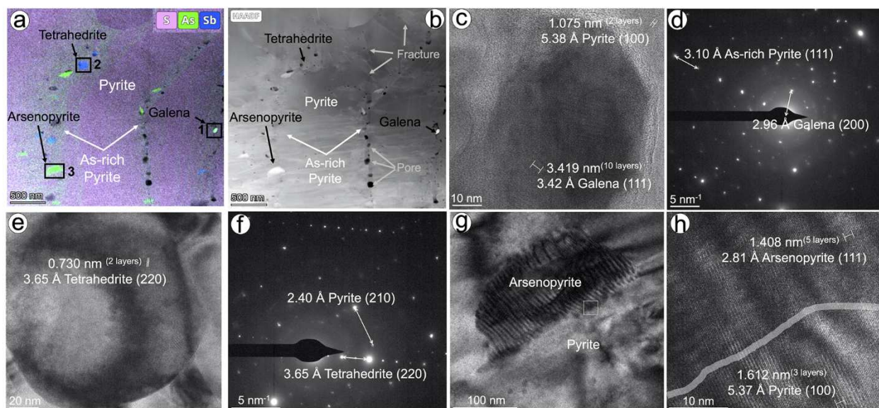
Fig. 5. Nanostructure of a selected area of the thin-foil #1 showing coexistence of nanoscale chemical zoning and metal-bearing NPs. TEM-EDS elemental and negative HAADF image of the selected area are shown in (a) and (b) respectively, whereas high magnification TEM images and corresponding SAED of NPs (galena, tetrahedrite and arsenopyrite) and host pyrite matrices are shown in (c-h). Black rectangles with numbers inset in (a) correspond to those NPs of galena (1), tetrahedrite (2) and arsenopyrite (3) shown in (c-h).
