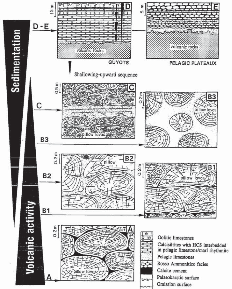
Fig. 2.- Normal o gradual types A to E, disposed according to the importance of volcanism against sedimentation. These different kinds of relationships models between the analysed pelagic and volcanic rocks are obtained from photographs and sketches drawn on the studied outcrops. They are described in the text and synthesized in table 1. Also two models of fossilization of the volcanic edifices (guyots and pelagic plateaux) are included (Types D and E).
