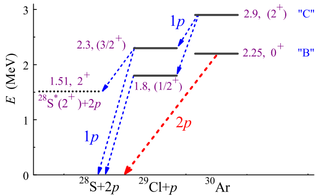
FIG. 5 (color online). Proposed decay scheme of low-lying ^{30}\text{Ar} and ^{29}\text{Cl} states, whose energy is given relative to the 2p and 1p thresholds, respectively. The assigned levels 0^+ and (2^+) in ^{30}\text{Ar} correspond to the peaks B and C in Fig. 2(c), respectively. The peak A in Fig. 2(c) comes from the ^{30}\text{Ar}^*(2^+) state, which decays into the excited state ^{28}\text{S}(2^+) by sequential 1p emissions via ^{29}\text{Cl}^*(3/2^+) .
