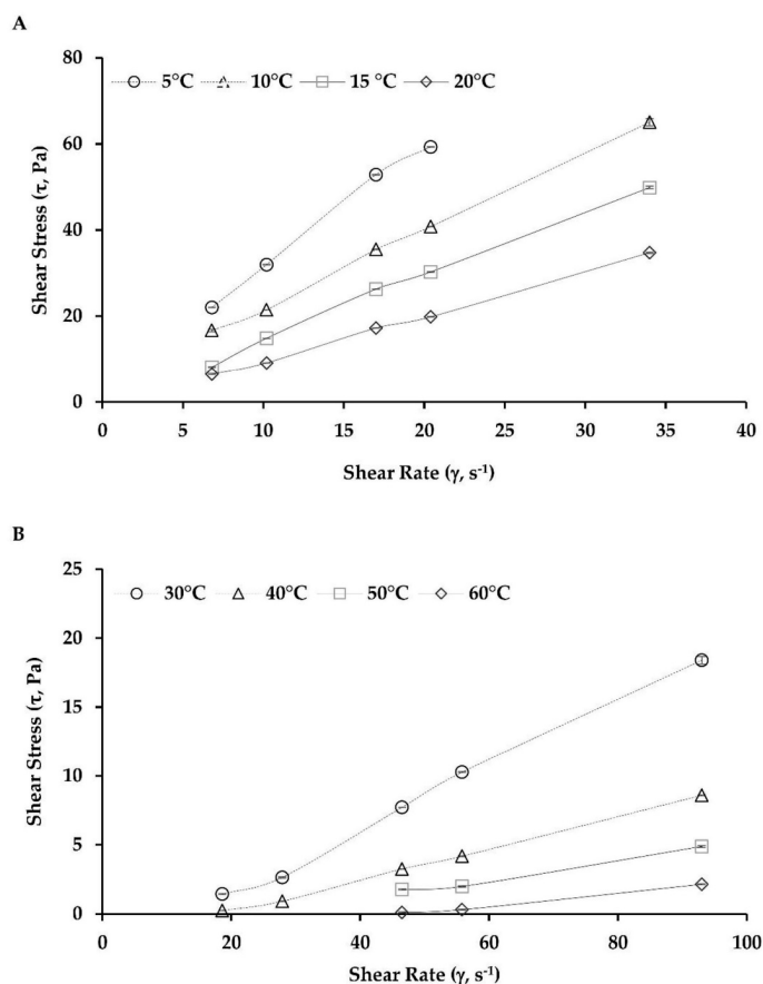
Figure 2. Rheogram flow curve of oleoresin at different temperatures with a relationship between shear stress ( \tau ; Pa) and shear rate ( \gamma ; s -1 ). (A) Low temperatures from 5 to 20 °C (with spindle SC-21; n = 3 ) and (B) high temperatures from 30 to 60 °C (with spindle SC-27; n = 3 ).
