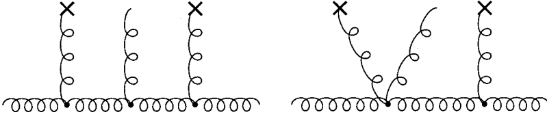
FIG. 1. Diagrams contributing to the tree-level Wilson coefficient in Eq. (7) Crosses mark the soft-gluon legs coming from the condensate.
