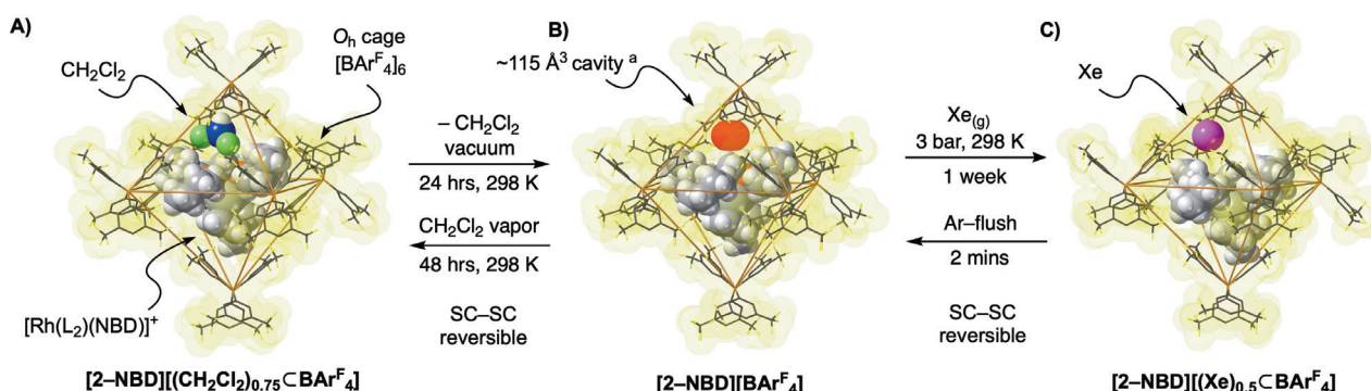
Figure 3. Synthesis and solid-state structures of A) [2-NBD][ (\text{CH}_2\text{Cl}_2)_{0.75}\text{C}\text{BAR}^{\text{F}}_4] , B) [2-NBD][ \text{BAR}^{\text{F}}_4] and C) [2-NBD][ (\text{Xe})_{0.5}\text{C}\text{BAR}^{\text{F}}_4] , and reversible encapsulation of guest \text{CH}_2\text{Cl}_2 and Xe via gas/solid SC–SC transformations. \text{L}_2 = \text{Cy}_2\text{PCH}_2\text{PCy}_2 . Molecular structures show the host \approx O_h - [\text{BAR}^{\text{F}}_4]^- cages using van der Waals radii. [a] Cavity as calculated using the contact surface with Mercury CSD software package at a probe radius of 1.5 Å and the grid spacing 0.2 Å. See the Supporting Information for displacement ellipsoid plot and further details.
