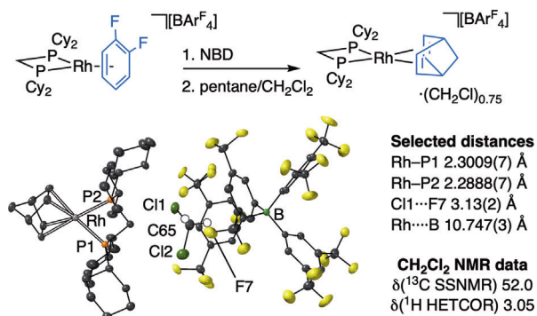
Figure 2. Synthesis of [2-NBD][ (\text{CH}_2\text{Cl}_2)_{0.75}\text{C}\text{BAR}^{\text{F}}_4] and structure of the cation, proximal anion and confined \text{CH}_2\text{Cl}_2 (major component).
