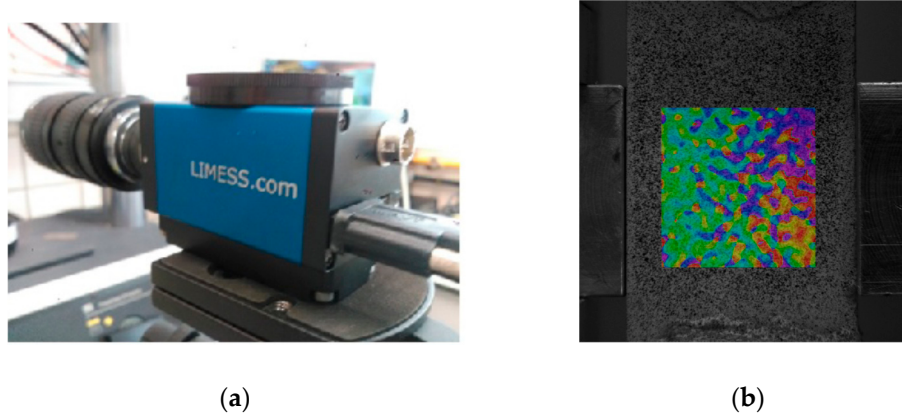
Figure 3. (a) Non-contact two-dimensional (2D) deformation system used to obtain the strain maps in the bone samples; (b) strains measured in the region of interest of the sample.
