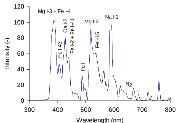
Figure 6. Main emission lines identified in the spectrum.
