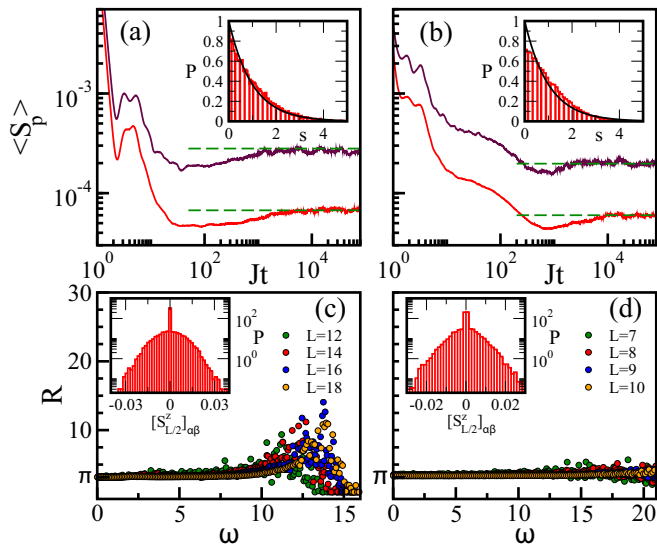
FIG. 3. Mean survival probability for the chaotic NNN spin-1/2 model [Eq. (7)] with L = 16, 18 (a) and for the spin-1 model with L = 9, 10, d = 0 , and \epsilon_1 = 0.05 (b). The horizontal line marks the saturation point. The insets show the corresponding level spacing distributions, L = 14 (a) and L = 8 (b). The ratio R(\omega) is shown for the NNN model (c) and for the spin-1 model (d) for different system sizes. The insets show the distributions of \langle \psi_\alpha | S_{L/2}^z | \psi_\beta \rangle for 200 eigenstates in the middle of the spectrum, L = 16 (c) and L = 9 (d). In (a) and (c): \sum_k S_k^z = 0 .
