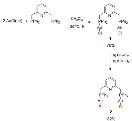
Scheme 2 Synthesis of complexes DPPMPY(AuCl) 2 , 1 , and DPPMPY(AuBr) 2 , 2 .
