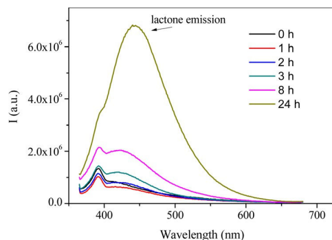
Fig. 5 Emission spectra of the catalytic reaction using complex 3 as a catalyst at different times. Experimental conditions: 70 °C, acetonitrile, Selectfluor (1.5 equivalents) and 3 (3%).
