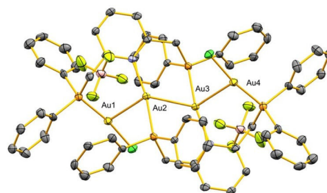
Fig. 3 Crystal structure of complex [(DPPMPY) 2 (Au 4 Cl 2 )](BF 4 ) 2 , 5. Hydrogen atoms are omitted for clarity. Structure (a) with the BF 4 - anion and (b) with the BF 4 - anion are omitted. Selected bond distances (Å) and angles (°): Au1–Au2, 3.288(0); Au2–Au3, 2.9904(9); Au3–Au4, 3.288(3); Au1–Au2–Au3, 95.7(1); Au2–Au3–Au4, 95.6(0).
