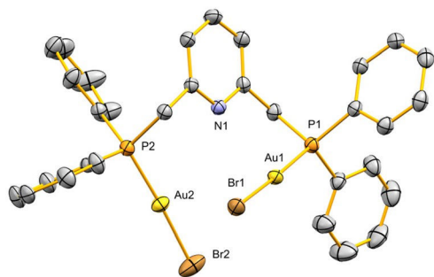
Fig. 2 Crystal structure of the complex DPPMPY(AuBr) 2 , 2. Hydrogen atoms and dichloromethane molecules are omitted for clarity. Selected bond distances (Å) and angles (°): Au(1)–P(1), 2.239(1); Au(2)–P(2), 2.232(1); Au(1)–Br(1), 2.4128(6); Au(2)–Br(2), 2.4057(7); Br(1)–Au(1)–P(1), 176.30(3); Br(2)–Au(2)–P(2), 176.51(4).
