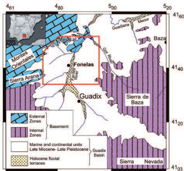
Fig. 1.- Location of the Guadix Basin in the Betic Cordillera (S. Spain). A square delimits the study area.
