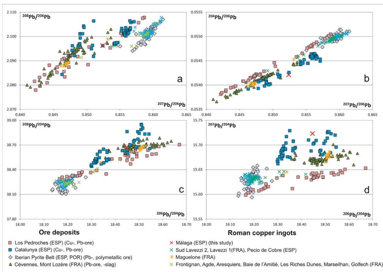
Figure 6. Diagrams with different lead isotope ratios. Ore and copper ingot data: Brévart et al. , 1982; Stos-Gale et al. , 1995; Canals i Cardellach, 1997; Lescuyer et al. , 1998; Marcoux, 1998; Pomiès et al. , 1998; Santos-Zalduegui et al. , 2004; Rico et al. , 2005; Baron et al. , 2006; Klein et al. , 2007, 2009; Rovira et al. , 2013 (M. Bode).
