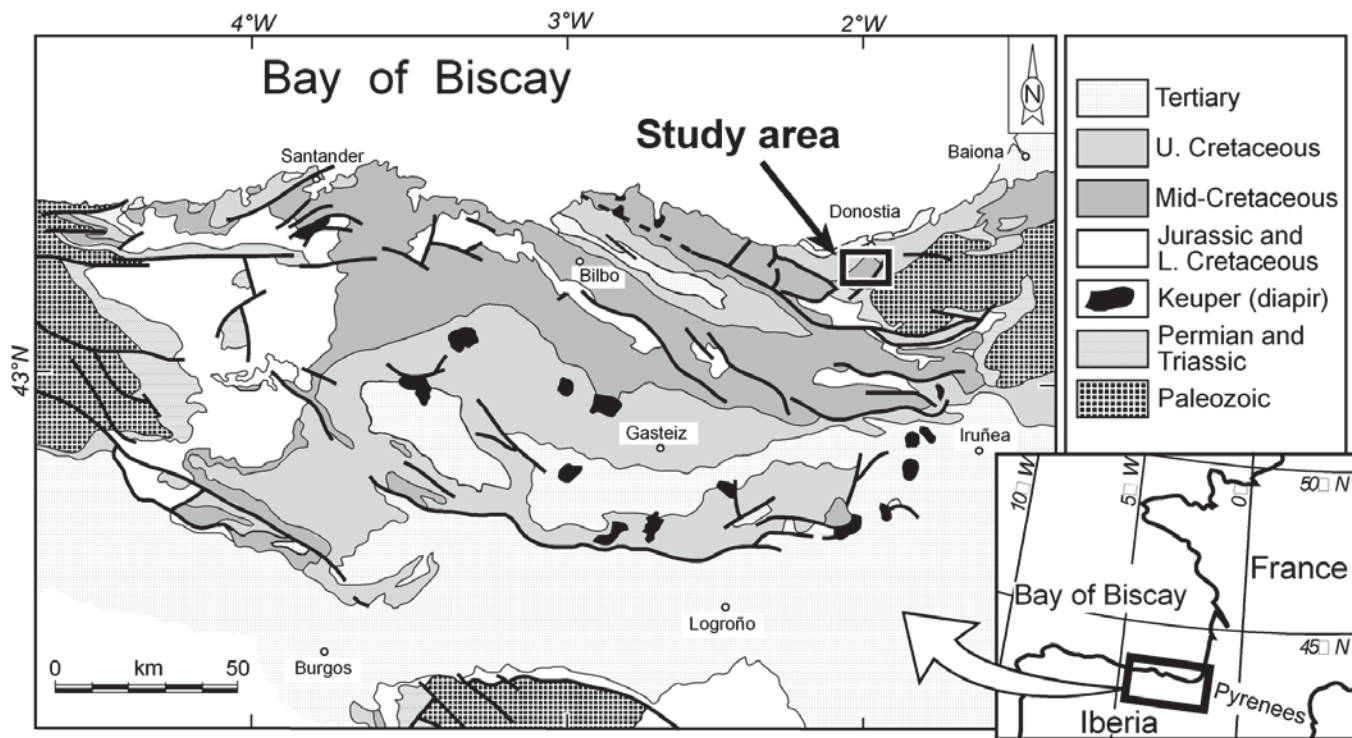
Fig. 1.- Geological map of the Basque-Cantabrian Basin with location of the study area.
