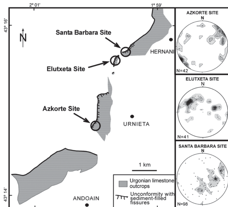
Fig. 2.- Outcrop map of Urganian platform limestones and location of the Azkorte, Elutxeta and Santa Barbara sites. Detail shows equal area density contour plots of sediment-filled fissures after removing of bedding dip (Confidence Index: 2.0%/1% area).
