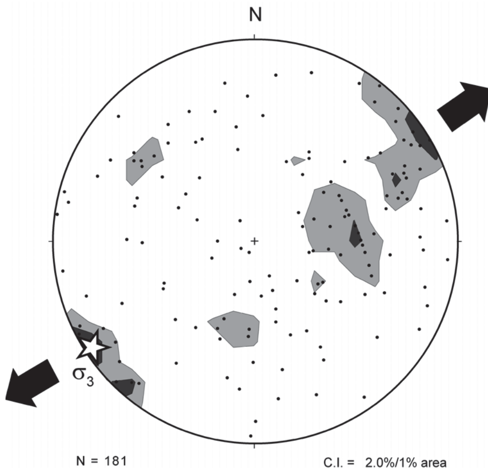
Fig. 4.- Equal area density contour plot of the Azkorte, Elutxeta and Santa Barbara sites fissure data. Star indicates minimum principal paleostress axis and the arrows extension direction.
