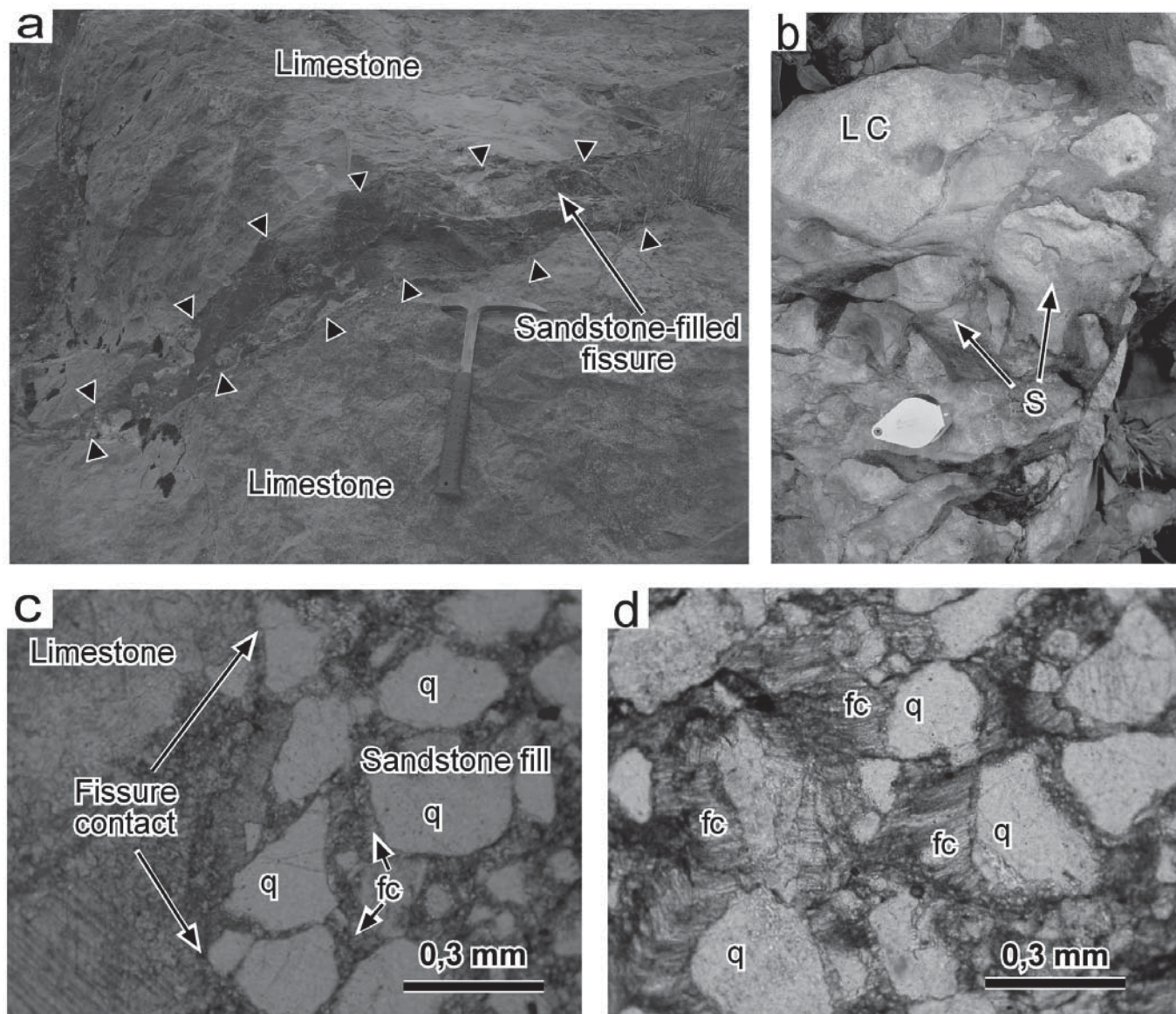
Fig. 3.- (a) Common aspect of sandstone-filled fissure; (b) Limestone breccia and sandstone fill (LC: limestone clast; S: sandstone); (c) Microphotograph of host limestone fissure contact and sandstone fill (fc: fibrous calcite; q: quartz); (d) Microphotograph of sandstone fill showing fibrous calcite cements (fc: fibrous calcite; q: quartz).
