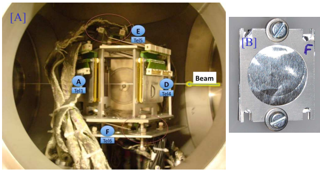
Fig. 1. [A] Picture of experimental setup used for the detection of the charged particles produced in the ^8\text{He}+^{208}\text{Pb} collisions (see text for details) [B] Picture of the fusion stack which was placed downstream of the scattering chamber in a separate chamber.
