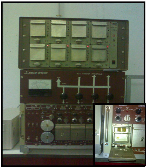
Fig. 3. Picture of measurement system at the Radiochemistry laboratory at the University of Huelva. In the inset, the detector and the sample holder can be seen.
