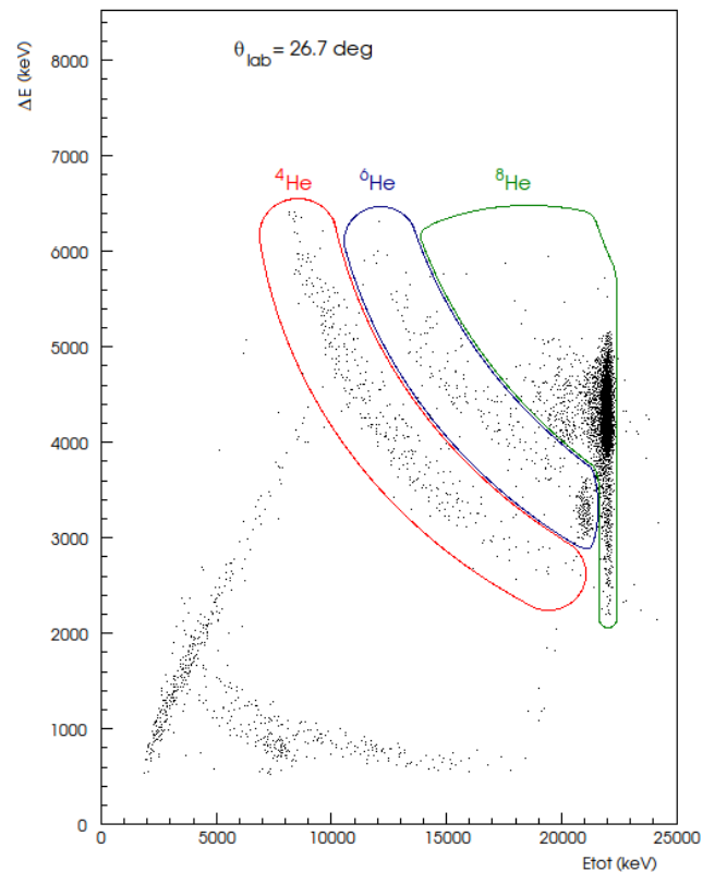
Fig. 2. A typical two dimensional spectrum of \Delta E vs. Etot for ^8\text{He}+^{208}\text{Pb} reaction measured at E_{\text{lab}} = 22 MeV and \theta_{\text{lab}} = 26.7^\circ . Different isotopes of 'He' can be easily identified in this telescope.
