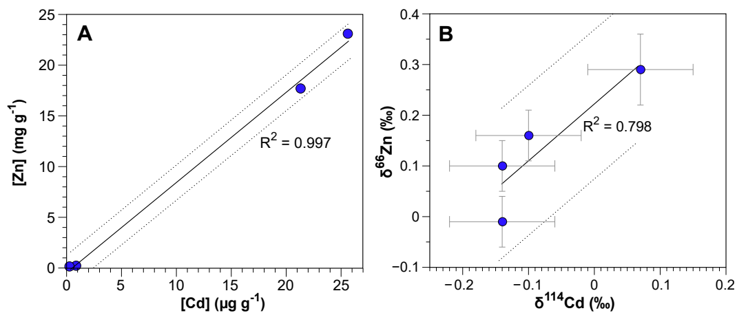
Fig. 7. Cross plots of concentration and isotopic data for mine sulfide rock samples. Panel A: Cd concentration versus Zn concentrations. Panel B: \delta^{114}\text{Cd} and \delta^{66}\text{Zn} values. The data are for four sulfide samples from the mines Tharsis (two samples), Corta Atalaya and San Telmo (TH1, TH2, CA, ST). Linear regression lines and 95% confidence intervals are shown for reference.
