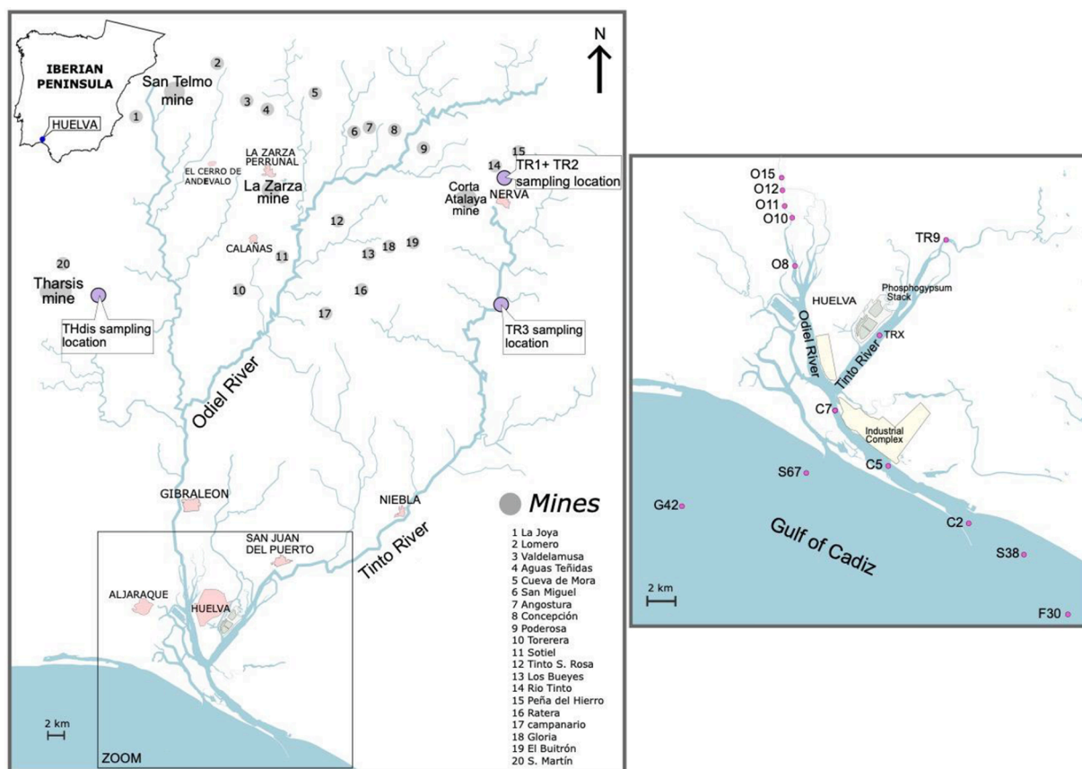
Fig. 1. Left: location of water sampling locations in the Odiel and Tinto River watersheds. Right: Zoom of Huelva region to show water sampling locations in the Ria of Huelva estuary and the Gulf of Cadiz. Some local towns are indicated in pink, the industrial complexes in the region are coloured yellow and the grey circles mark the main mine localities (not an exhaustive list).
