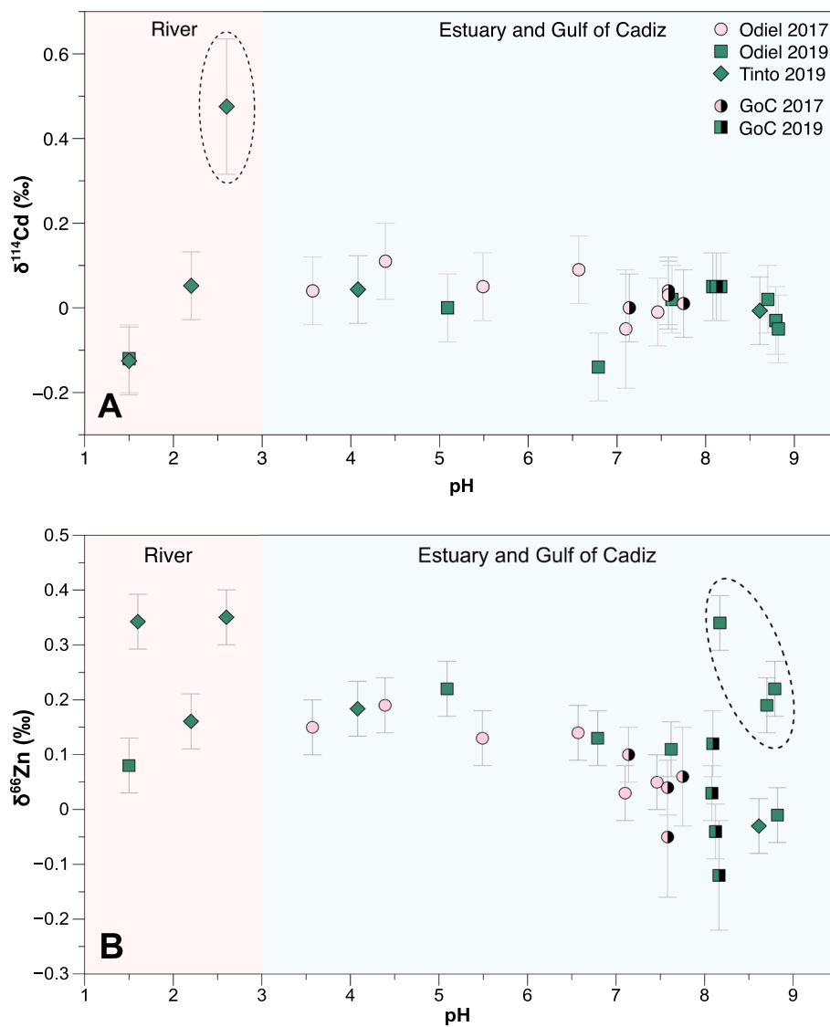
Fig. 6. Cd (Panel A) and Zn (Panel B) isotope compositions plotted against pH for the water samples collected in 2017 and 2019. Colour shading and symbols are as in Fig. 5. Samples from the confluence of the estuary are included in the ‘Odiel’ datasets. The ‘Tinto’ samples include waters collected in the Tinto River and Tinto branch of the Ria of Huelva estuary. Samples with anomalous \delta^{114}\text{Cd} and \delta^{66}\text{Zn} values are circled (see text for discussion).
