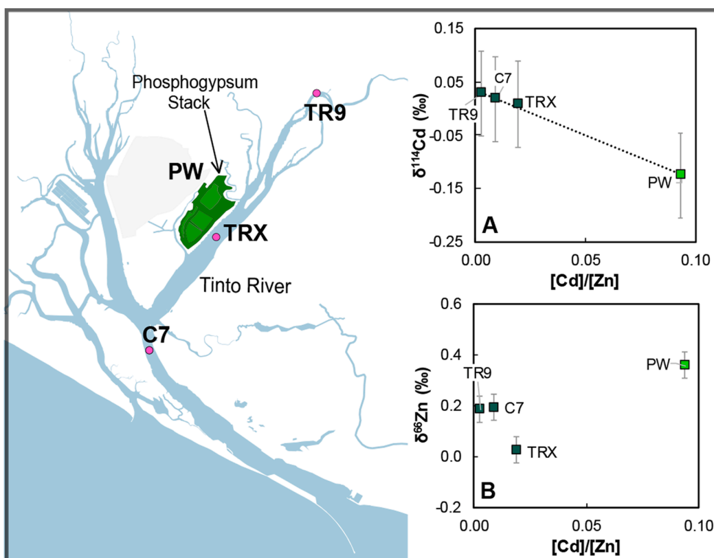
Fig. 9. Map of the Ria of Huelva estuary showing the location of the phosphogypsum stack and locations of relevant samples. PW refers to process water, which is the solution sitting on the surface of the phosphogypsum stack (coloured in a lighter green). Inset graphs show dissolved \delta^{114}\text{Cd} (Panel A) and \delta^{66}\text{Zn} (Panel B) versus the ratio of dissolved Cd/Zn concentration. Dashed line on Panel A shows a linear regression, showing the likely impact of Cd contamination from the phosphogypsum stack on Cd/Zn ratios and \delta^{114}\text{Cd} values in the estuary.
