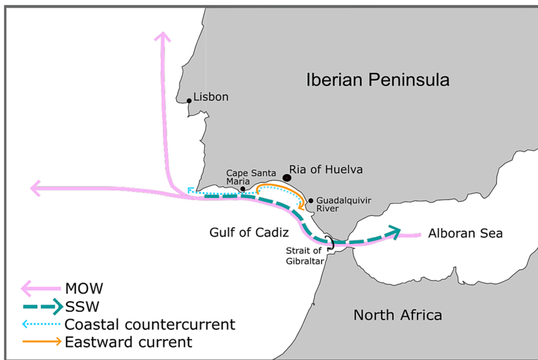
Fig. 10. Schematic representation of relevant currents in the Gulf of Cadiz. Spanish Shelf Water (SSW) is a surface current, whilst the flow of Mediterranean Outflow Water (MOW) is at depths of 400 m in the Gulf of Cadiz and sinks to between 500 and 1500 m along the western coast of the Iberian Peninsula. The black curly arrow in the Strait of Gibraltar demonstrates proposed coupling between the inflow and outflow water masses (Peliz et al., 2009).
