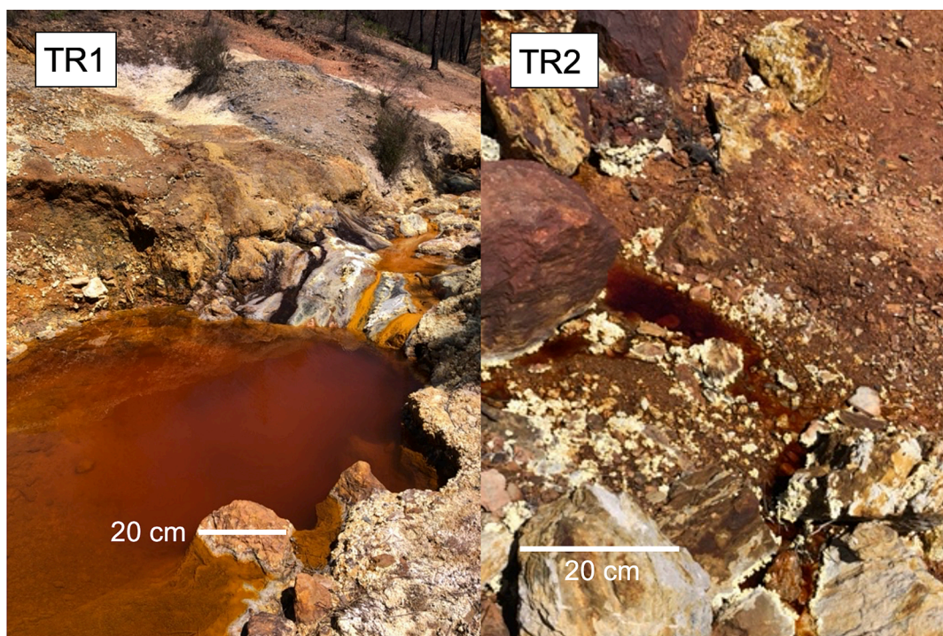
Fig. 2. Photographs of the sampling locations of TR1 and TR2, showing distinctive impact of AMD (dark red colour) at TR2 compared to the lighter orange at TR1, indicative of schwertmannite precipitation.
