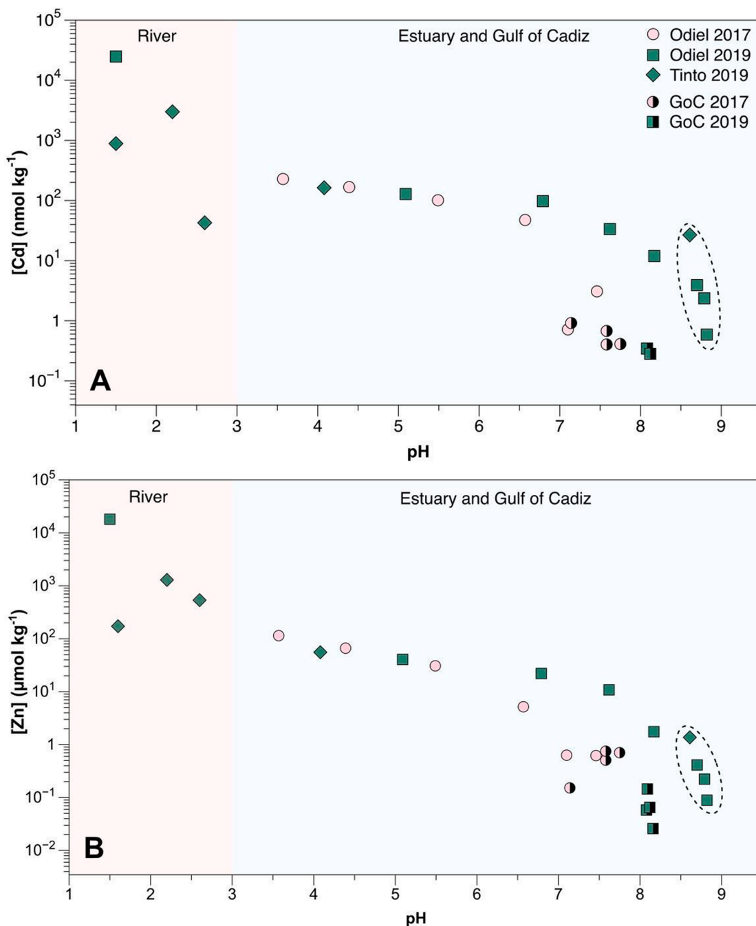
Fig. 5. Dissolved Cd (Panel A) and dissolved Zn (Panel B) concentrations against pH for the Odiel and Tinto River watersheds (orange shaded background) and for the Ria of Huelva estuary and Gulf of Cadiz (blue shaded background), for samples collected in May 2017 and June 2019. Samples from the Gulf of Cadiz (GoC) are those with symbols divided in half. Samples from the confluence of the estuary are included in the ‘Odiel’ datasets. The ‘Tinto’ samples include waters collected in the Tinto River and Tinto branch of the Ria of Huelva estuary. Circled datapoints are 2019 estuarine samples with pH values more alkaline than Gulf of Cadiz seawater (see text for discussion).
