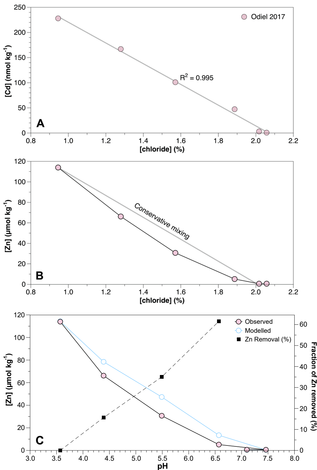
Fig. 8. The behaviour of Cd and Zn in the Odiel branch of the Ria of Huelva estuary in 2017. Panel A: Cd (black line, pink circles) versus chloride concentrations with a linear regression function (grey line) including R^2 value, illustrating conservative behaviour of Cd in the estuary in 2017. Panel B: Zn versus chloride concentrations, showing non-conservative behaviour of Zn in the estuary in 2017. Panel C: Zn concentrations versus pH compared to modelled Zn concentrations assuming conservative behaviour (blue line, open circles). Also shown is the modelled fraction of Zn removed from the dissolved phase (dashed black line, see text for discussion).
