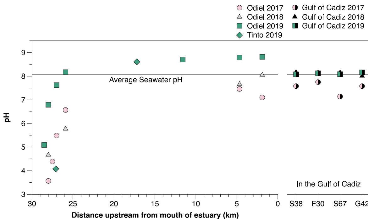
Fig. 4. pH plotted against distance upstream from the mouth of the Ria of Huelva estuary and for the Gulf of Cadiz in 2017, 2018 and 2019.
