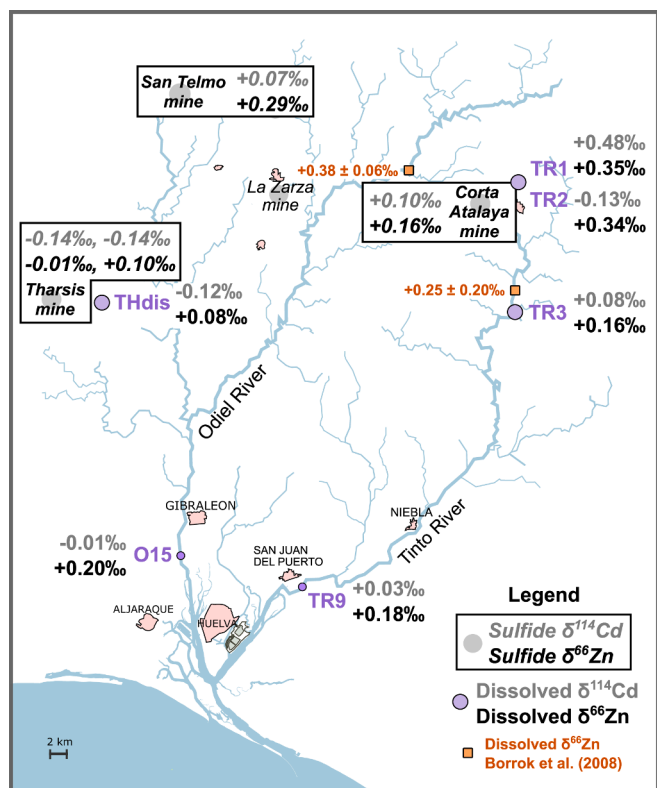
Fig. 3. \delta^{114}\text{Cd} (grey text) and \delta^{66}\text{Zn} (black text) values of selected samples collected in the Odiel and Tinto watersheds in 2019. Boxed \delta -values in bold italic font are for digests of mine sulfide samples. \delta -values in bold font are for dissolved phase water samples. Orange squares and values give the locations and \delta^{66}\text{Zn} values of water samples reported in Borrok et al. (2008).
