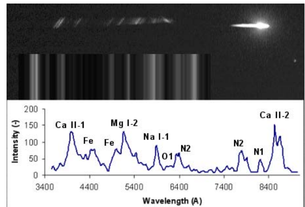
Figure 3. Raw and processed emission spectrum of the SPMN140111 Comae Berenicids fireball.
