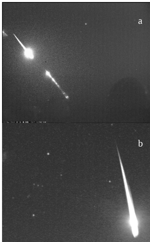
Figure 1. Mag. -8 Comae Berenicids fireball imaged from a) La Hita Astronomical Observatory b) La Murta Astronomical Observatory on Jan. 14, 2011, at 0h44m41.5 \pm 0.1s UT.
