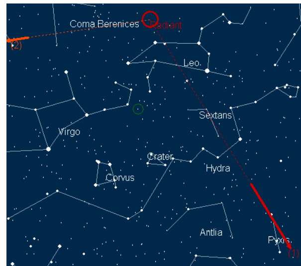
Figure 2. Radiant calculated by performing the astrometric calibration from two observing stations (1. La Hita, and 2. Arenosillo).
