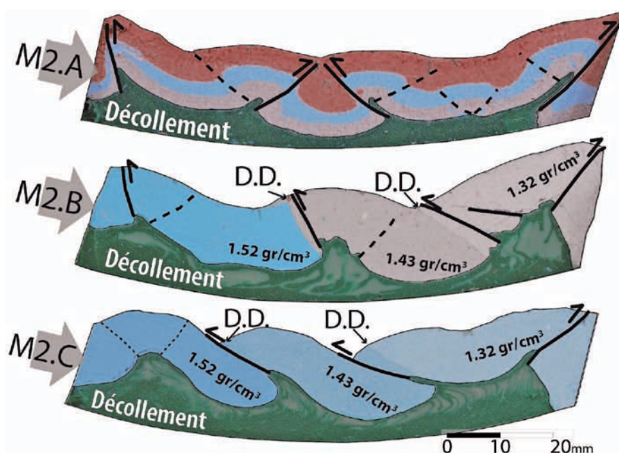
Fig. 2.- Interpreted cross-sections of compressional models. Density is indicated and density discontinuities (D.D.) displayed and labelled. See colour figure on the Web.
