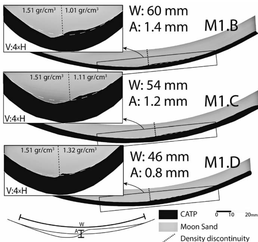
Fig. 1.- Interpreted sketches from cross-section at the end of experiments and detail of the structure that developed near the density discontinuity (vertically exaggerated). Dimensions of syncline-anticlines structures are characterized by their wavelength (W) and amplitude (A).
