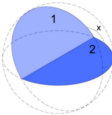
Figure 4. Two half-disks with equal radius R, sharing their diameters for any angle of X^\circ degrees.
