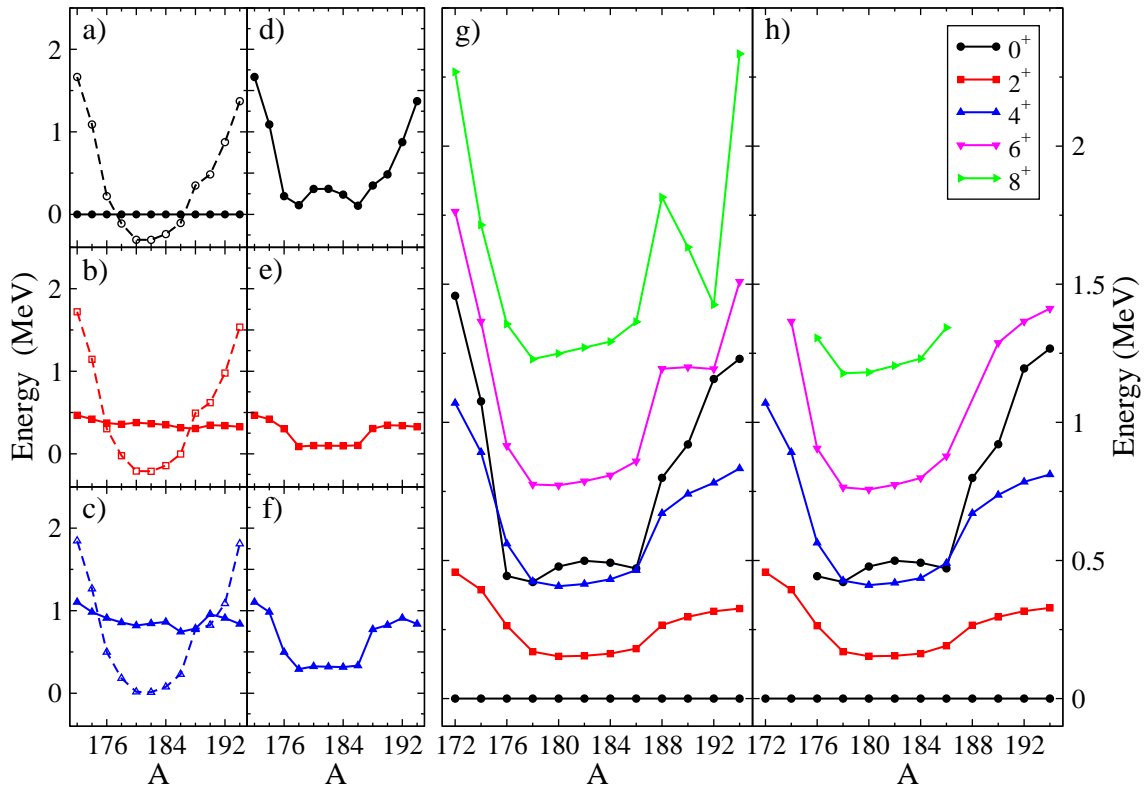
FIG. 11: (Color online) Energy systematic of the unperturbed (IBM-CM) first regular and intruder states (full line for regular, while dashed line for intruder states in panels a), b), and c)), a) 0_{1,2}^+ energies relative to the energy of the 0^+ regular state, b) 2_{1,2}^+ energies relative to the energy of the 0^+ regular state, c) 4_{1,2}^+ energies relative to the energy of the 0^+ regular state, d) 0_2^+ energies relative to the energy of the 0_1^+ state, e) 2_1^+ energies relative to the energy of the 0_1^+ state, f) 4_1^+ energies relative to the energy of the 0_1^+ state. Panel g) corresponds to the full (including now all states) IBM-CM calculation and panel h) shows the experimental data of the yrast band states plus the 0_2^+ state.
