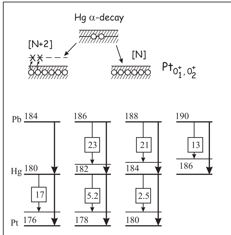
FIG. 13: A schematic view of the \alpha -decay proceeding from the 0^+ Hg ground state in the 0^+_{1,2} states in the Pt nuclei. The inset boxes present the experimental \alpha decay hindrance factors, which were taken from [22–24] and from Nucl. Data Sheets.
