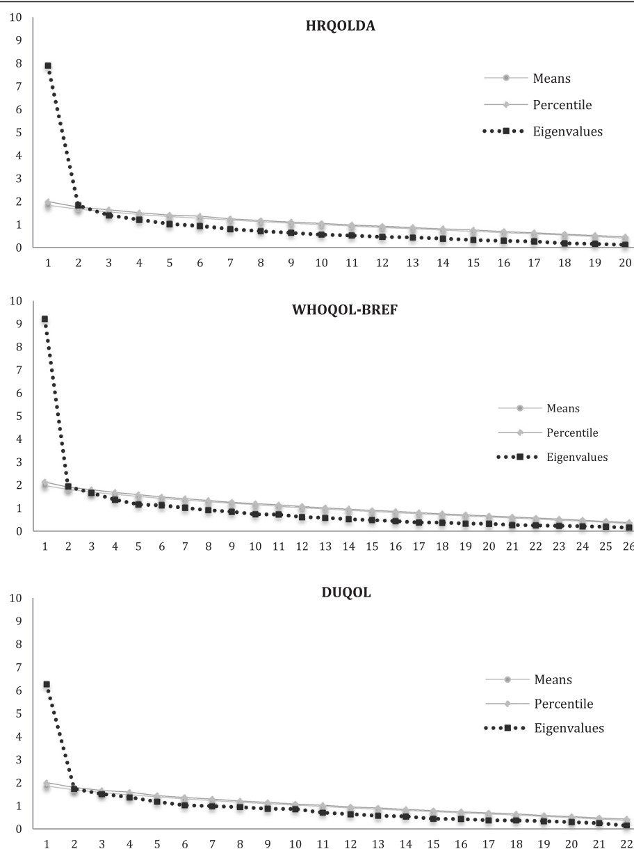
Fig. 1 Parallel analysis graphics of HRQOLDA, WHOQOL-BREF and DUQOL
