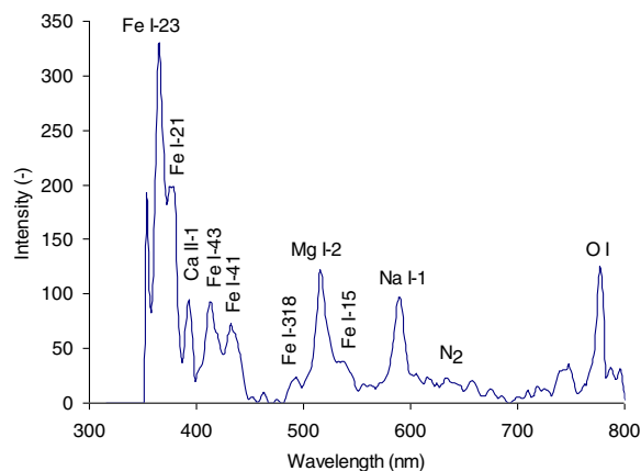
Figure 5 Calibrated emission spectrum of the Geminid fireball discussed in the text. Intensity is expressed in arbitrary units.
