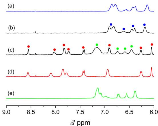
Figure 3. Partial ^1\text{H} NMR spectra of (a) dye 1 at pH 7.6, (b) dye 1 in presence of CB7 and amine 2 at pH 7.6, (c) dye 1 in presence of CB7 and amine 2 at pH 5.0, (d) dye 1 in presence of CB7 at pH 5.0, and (e) dye 1 at pH 5.0. Concentrations: [\mathbf{1}] = 0.93 \text{ mM} , [\mathbf{2}] = [\text{CB7}] = 1.0 \text{ mM} . The coloured dots in (b) and (c) show the assignments of the signals to free and complexed dye at the different pH values, based on the comparison with the colour-matching spectra in (a), (d), and (e).
