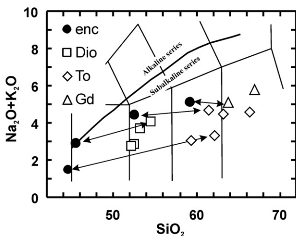
FIGURE 2 | Total alkalis versus \text{SiO}_2 diagram for the Valle Fertil granitoids and their enclosed microgranular enclaves. Granitoids display a typical subalkaline trend. Arrows connect the composition of each analyzed inclusion with its host granitoid.
