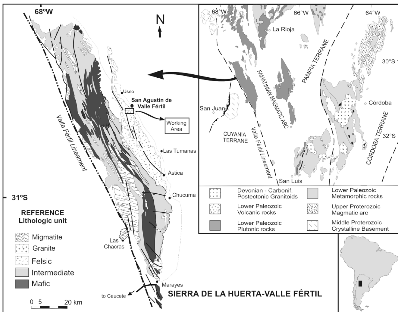
FIGURE 1 | Simplified geologic map of the Sierras de Valle F rtil – La Huerta taken after the geological maps of Mirr  (1976). The larger inset shows the geological map of the Famatinian paleo-magmatic arc with the distribution of major lithostratigraphic units.
