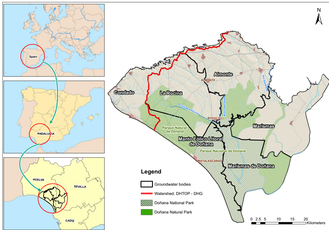
Fig. 1 The Almonte-Marismas aquifer system underlying Doñana, the division between six groundwater bodies, and the areas protected within Doñana National and Natural Parks (which, combined, make up “Doñana Natural Space”)
