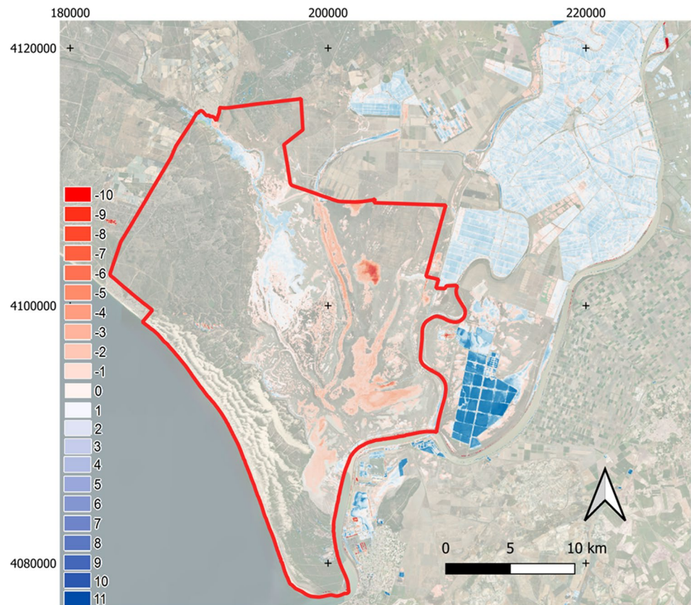
Fig. 3 Theil–Sen slope in days/year showing the hydroperiod trend from 1974 to 2021. Red indicates consistent and significant decreasing trend in hydroperiod, while blue indicates the opposite (methods from Díaz-Delgado et al. 2016). The boundary of Doñana National Park is shown in red
