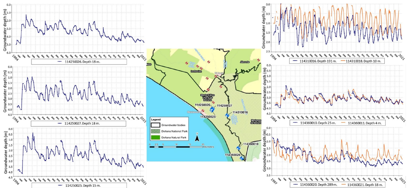
Fig. 2 Temporal piezometric evolution of groundwater levels in the dune ponds (graphs on the left side) and three sites in the west ecotone (right side) in Doñana. The declines in depth shown in each graph are stronger in those piezometers closer to areas of ground-
