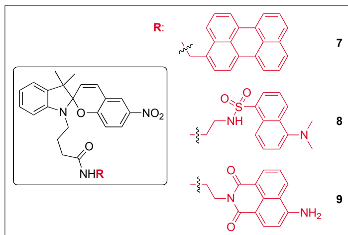
Fig. 6. Spiropyran 7–9 with appended fluorophores for photochromic switching of energy transfer.
