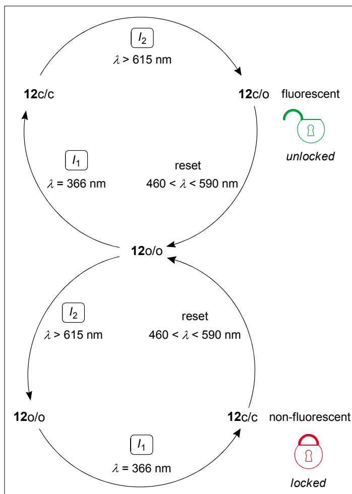
Fig. 10. Structure of the fluorescent 12c/o form of the multiphotochromic platform 12 and network of photochemical transformations of the system.
