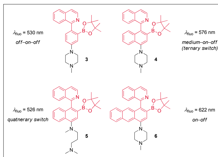
Fig. 4. Structures of fluorescent borylated arylisoquinolines (BAI dyes) 3–6 for multi-level switching.
