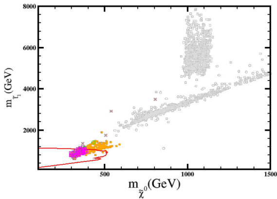
FIGURE 5 | As in Figure 3 for the m_{\tilde{t}_1} vs. m_{\tilde{\chi}_0} scatter plot.
