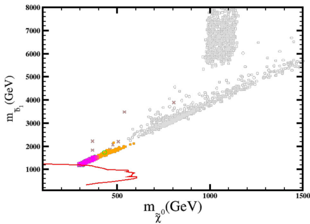
FIGURE 6 | As in Figure 3 for the m_{\tilde{b}_1} vs. m_{\tilde{\chi}_0} scatter plot.
