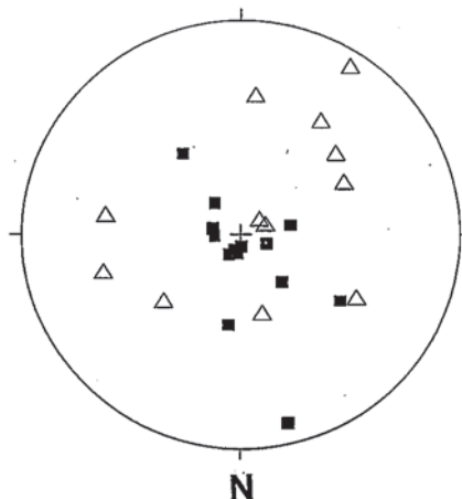
Fig. 3- Right-dihedra diagrams for the Agrón earthquake series. A, all earthquakes (16 earthquakes). B, focal mechanisms of m>2.5 earthquakes (11 earthquakes). C, focal mechanisms of normal faults with m>2.5 (8 earthquakes). D, focal mechanisms of reverse faults with m>2.5 (3 earthquakes). E, focal mechanisms of earthquakes with m≤2.5 (5 earthquakes). Software, G. de Vicente.
