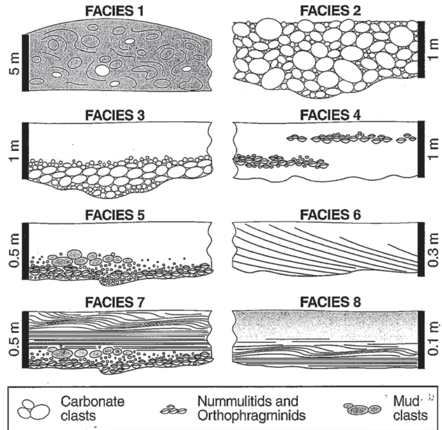
Fig. 3.- Sketch of the main characteristics of the eight facies recognized in the calciclastic deposits. Explanation within the text.
