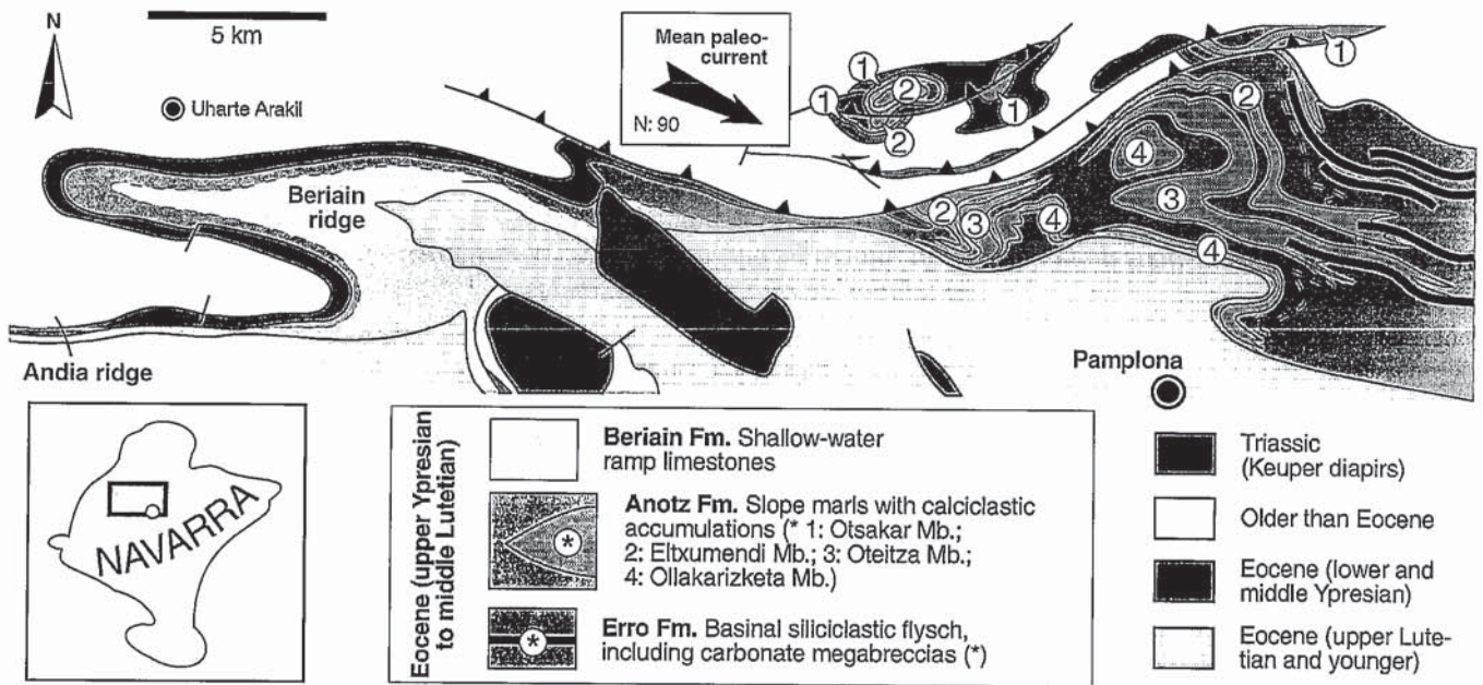
Fig. 1.- Geological map of the study area showing the four calciclastic members in the Anotz Fm (north of Pamplona) and their mean paleocurrent vector.
