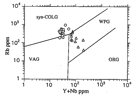
Fig. 4.- Diagram Rb vs. Y+Nb for the geodynamic classification of granitoid rocks ( Pearce et al , 1984). Symbols: circles = type 1 meta-granites and ortogneisses; triangles = type 2 ortogneisses
