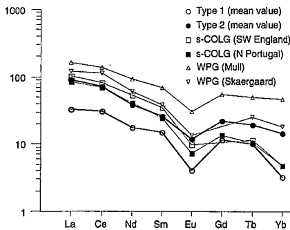
Fig. 3.- Chondrite-normalized REE patterns of mean values of type 1 meta-granites and ortogneisses and type 2 ortogneisses, compared with granitoids from known geodynamic setting in: et al. , (1984) and Albuquerque, (1978).
