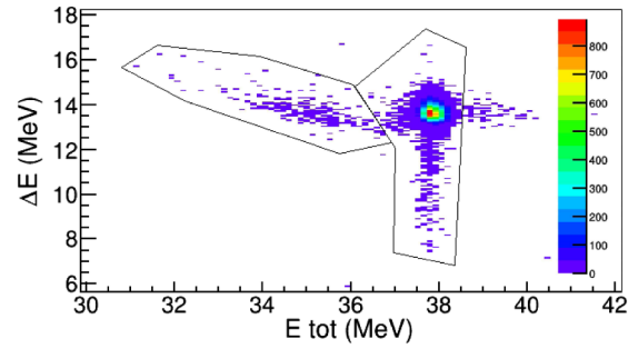
FIG. 1. Two-dimensional \Delta E - E_{\text{tot}} spectrum of the ^{11}\text{Be} + ^{197}\text{Au} reaction at E_{\text{lab}} = 39.6 MeV for a single pixel at \theta_{\text{lab}} = 18^\circ . The dominant feature corresponds to quasielastic, while the other locus corresponds to the ^{10}\text{Be} fragments detected after the breakup.
