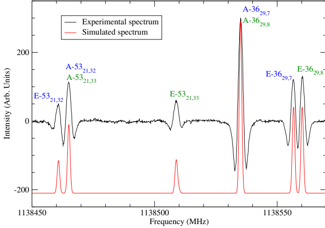
Fig. 1. Portion of the experimental spectrum recorded with the JPL experimental setup in the frequency range 1 138 450–1 138 570 MHz. The simulated spectrum is also provided by using the Hamiltonian parameter values given in Table 2 and the dipole moment components as explained in the text. The involved features are assigned as \Gamma - J_{K_a, K_c} for a transition to a state with J' = J - 1 , K'_a = K_a - 1 , and K'_c = K_c and with symmetry \Gamma (A or E). Transitions J = K_a + K_c are labeled in blue and J + 1 = K_a + K_c in green.
