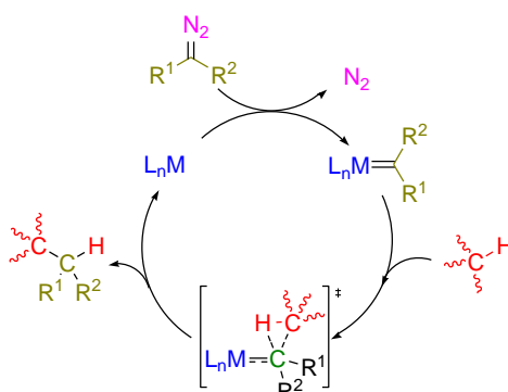
Scheme 1. C-H bond functionalization by metal-catalyzed carbene insertion from diazo compounds.
