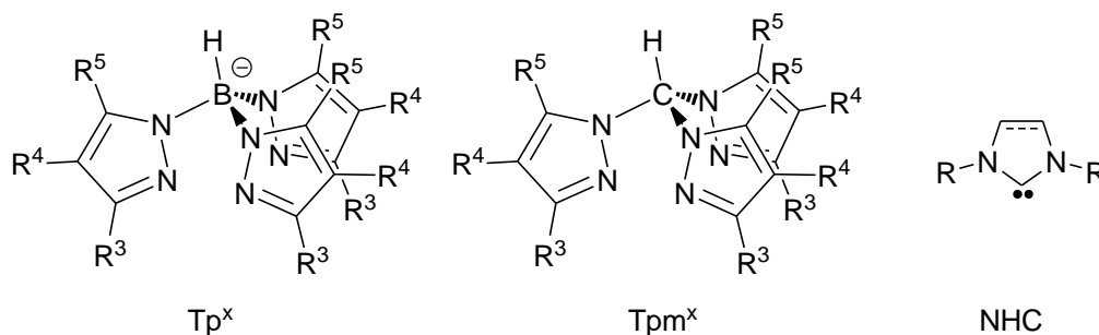
Figure 1. Some ligands employed in the coinage metals-catalyzed C-H bond functionalization by carbene insertion from diazo compounds.
