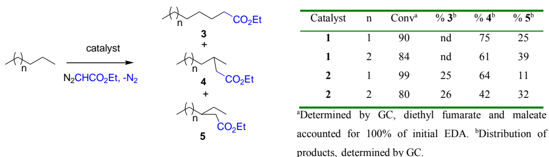
Scheme 2. Functionalization of pentane and hexane with EDA and 1 or 2 as the catalyst.
