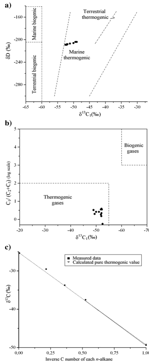
Fig. 3. a) and b), respectively, relationships of \delta\text{D} to \delta^{13}\text{C}_1 and of \delta^{13}\text{C}_1 to \text{C}_1/(\text{C}_2 + \text{C}_3) for the studied gases; c) \delta^{13}\text{C}
