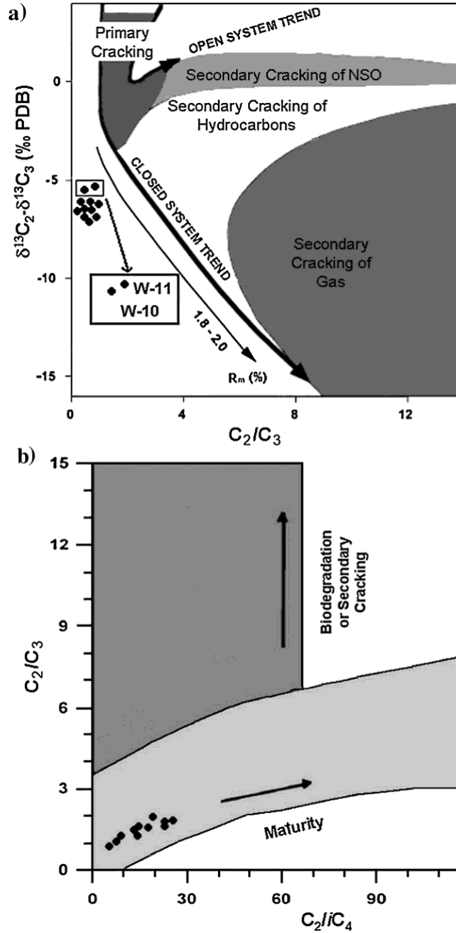
Fig. 5. a) and b), respectively, plots ( \delta^{13}\text{C}_2 - \delta^{13}\text{C}_3 vs. \text{C}_2/\text{C}_3 ) and ( \text{C}_2/i\text{C}_4 against \text{C}_2/\text{C}_3 ) for the gas samples.
