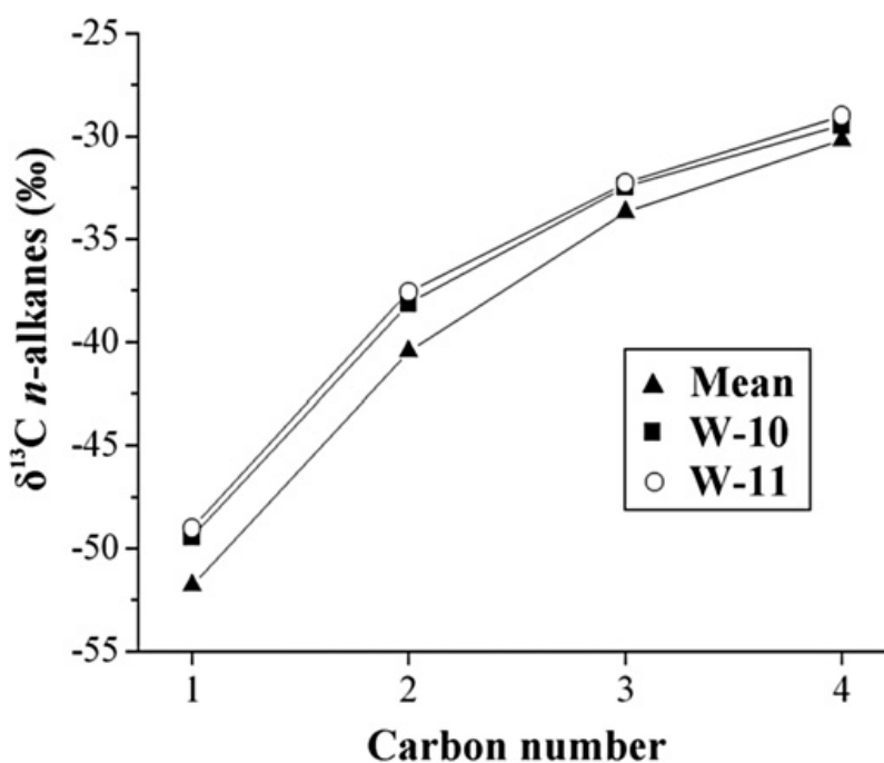
Fig. 4. \delta^{13}\text{C} values (‰) in methane, ethane and propane from W-10, W-11, and the mean of the remaining sampled gases.
