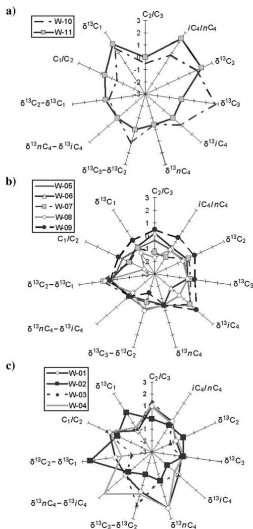
Fig. 6. a), b) and c), three normalized Gostar diagrams for the groups of gas samples coming from the studied reservoir. The scales are the same for all 11 axes of each diagram.
