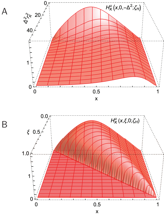
Fig. 3. (color online) Kaon. PTIR GPD obtained using Eq.(11) and the associated LFWF defined by Eqs. (5)-(7) and Table 1. Upper panel-A. H_K^u(x, \xi = 0, -\Delta^2; \zeta_H) . Lower panel-B. H_K^u(x, \xi, 0; \zeta_H) . Here, r_K = 0.56 fm, computed using Eq. (17). (Experiment [69, 73]: 0.560(31) fm, 0.53 fm, respectively.)
