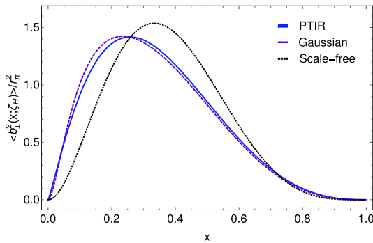
Fig. 9. (color online) \langle b_{\perp}^2(x; \zeta_H) \rangle_u^{\pi} / r_{\pi}^2 , Eq. (26): longitudinal light-front distribution of the mean-square transverse light-front extent of u -in- \pi . Results obtained with PTIR GPD, Sec. IV.A, and factorised GPD, Sec. IV.B, are compared with that characterising a scale-free system, whose valence DF is given by Eq. (27).
