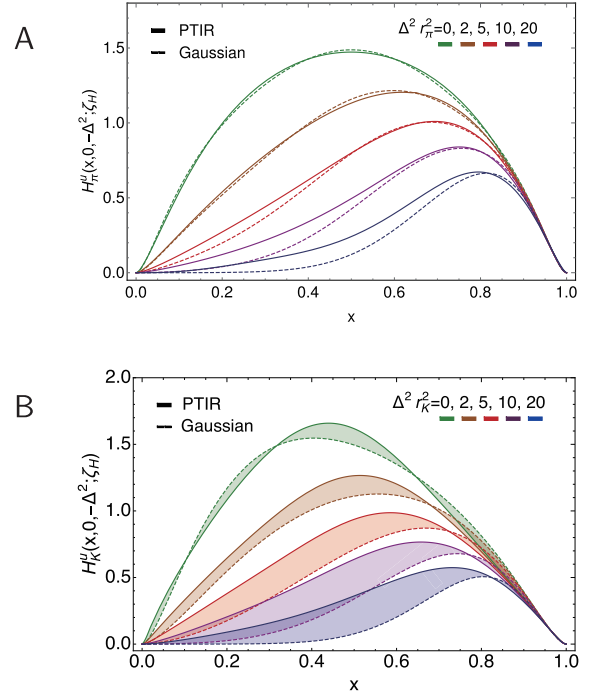
Fig. 6. (color online) Upper panel-A. u -in- \pi GPD, plotted as a function of x on contours of constant \Delta^2 r_\pi^2 : solid curves - produced using PTIR LFWF, Eqs. (5)-(7) and Table 1; and dashed curves - results from factorised LFWF, Eq. (23). Lower panel-B. Kindred curves for u -in- K GPD. The factorised kaon LFWF is obtained with d_K = 0.07 in Eqs. (20), (22). (Shading highlights curves that should be compared.)
