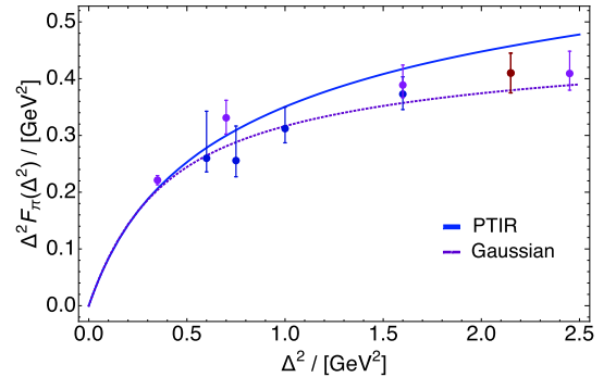
Fig. 7. (color online) \Delta^2 F_\pi(\Delta^2) obtained using the GPDs drawn in Fig. 2: PTIR (solid blue curve), Sec. IV.A; and factorised LFWF (short-dashed magenta), Sec. IV.B. Data from Refs. [75, 76].
