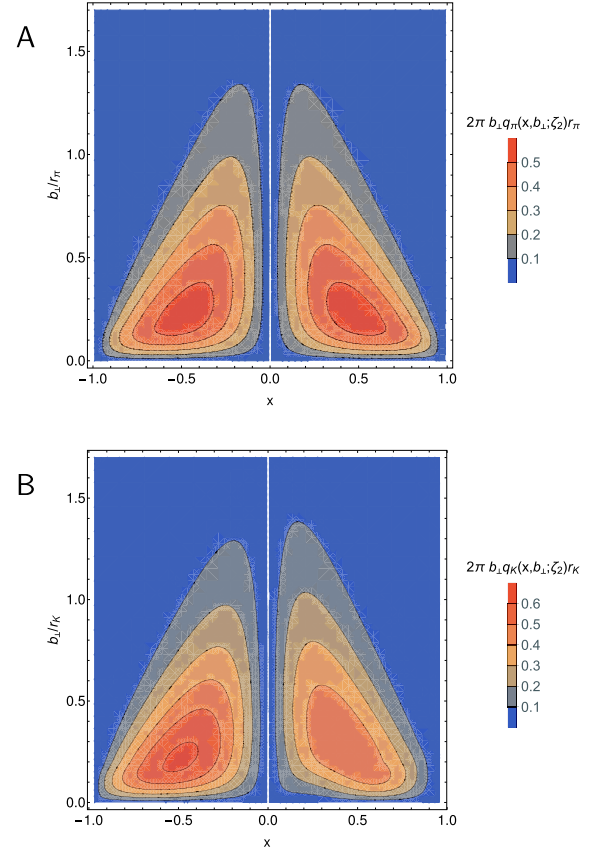
Fig. 19. (color online) Upper panel-A. Pion. IPS distributions for \bar{d} - (left) and u -quarks (right), charting the x -dependent probability density for locating these objects at distance |b_\perp| from the pion's centre of transverse momentum. Lower panel-B Kaon. Analogous profiles for \bar{s} and u -quarks in the K^+ . Curves calculated using the \zeta_{\mathcal{H}} \rightarrow \zeta_2 valence-quark GPDs drawn in Figs. 10A, 10B into the right-hand-side of Eq. (24) and its analogue for the \bar{s} -in-kaon.
