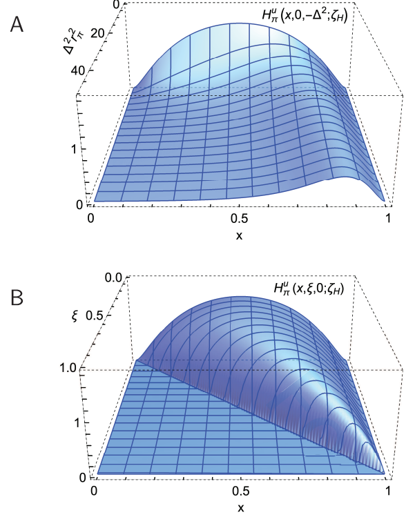
Fig. 2. (color online) Pion. PTIR GPD obtained using Eq.(11) and the LFWF in Fig. 1A. Upper panel-A. H_\pi^u(x, \xi = 0, -\Delta^2; \zeta_H) . Lower panel-B. H_\pi^u(x, \xi, 0; \zeta_H) . Here, r_\pi \approx 0.69 fm, computed using Eq. (17). (Experiment [69, 73]: 0.659(4) fm, 0.640(7) fm, respectively.)
