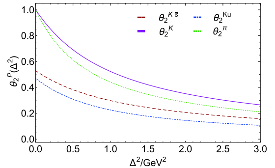
Fig. 12. (color online) Mass-squared distribution form factors, \theta_2 , for the pion and kaon, along with a \zeta = \zeta_{\mathcal{H}} flavour separation of the latter, all computed using Eq. (23) (based on factorised LFWF) in Eq. (33) and \xi = 0 .
