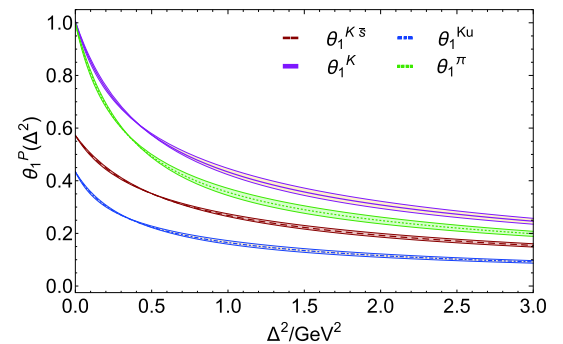
Fig. 13. (color online) Pressure distribution form factors, \theta_1 , for the pion and kaon, along with a \zeta = \zeta_{\mathcal{H}} flavour separation of the latter, all computed using Eq. (37) with \theta_2 from Fig. 12. The band associated with each curve describes the model uncertainty explained in connection with Eq. (37).
