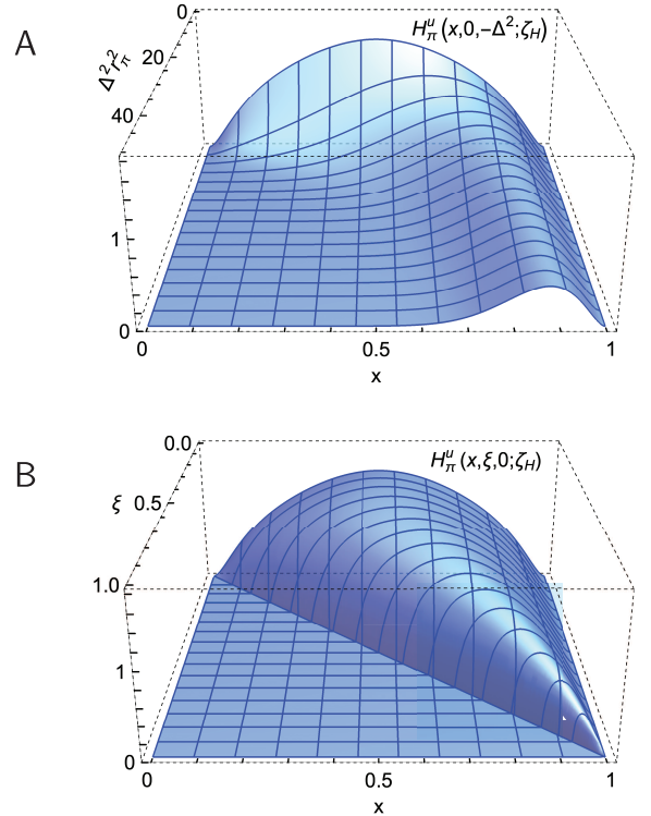
Fig. 4. (color online) Pion GPD obtained using Eq. (11) and the factorised LFWF discussed in Sec. IV.B. Upper panel-A. H_{\pi}^u(x, \xi = 0, -\Delta^2; \zeta_H) . Lower panel-B. H_{\pi}^u(x, \xi, 0; \zeta_H) .
