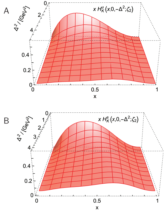
Fig. 18. (color online) Kaon GPDs ( \xi = 0 ) computed in Sec. IV.B, beginning with the factorised LFWF, evolved to \zeta_H \rightarrow \zeta_2 : Upper panel-A : u -valence; and lower-B : \bar{s} -valence.
