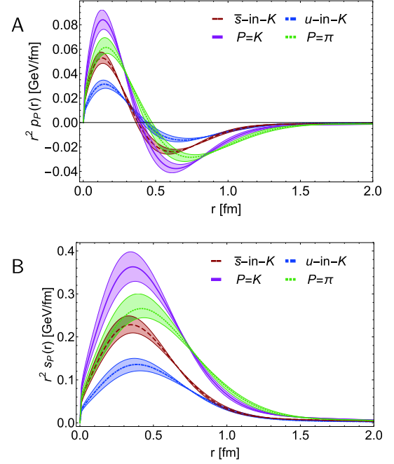
Fig. 15. (color online) Kaon profiles. Upper panel-A : pressure, Eq. (45a). Lower panel-B : shear force, Eq. (45b). K results obtained using Eq. (37), with M_u = M_u(1 \pm 0.1) , M_{\bar{s}} = M_{\bar{s}}(1 \pm 0.1) : solid magenta curve and band. Flavour separation: u -in- K - dot-dashed blue curve; and \bar{s} -in- K - dashed red. Dotted green curve and like-coloured band reproduce the pion profiles in Fig. 14.
