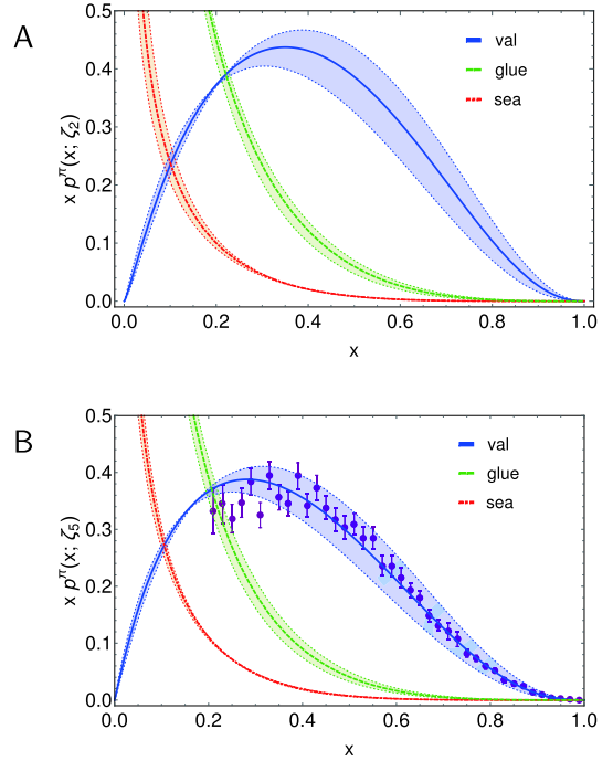
Fig. 16. (color online) Pion parton DFs obtained using Eqs. (67) to evolve the \zeta = \zeta_H valence-quark DF specified by Eq. (10) and the coefficients and powers listed in Table 2. Upper panel-A: \zeta_H \rightarrow \zeta_2 , seeded by \langle 2x \rangle_u^{\zeta_2} = 0.50(5) , producing \langle x \rangle_g^{\zeta_2} = 0.40(3) , \langle x \rangle_S^{\zeta_2} = 0.10(2) . Lower panel-B: \zeta_H \rightarrow \zeta_5 , seeded by \langle 2x \rangle_u^{\zeta_5} = 0.42(4) , producing \langle x \rangle_g^{\zeta_5} = 0.45(2) , \langle x \rangle_S^{\zeta_5} = 0.13(2) . No explicit choice for the effective charge was necessary to obtain these DFs. Data in Panel B: Ref. [43, E615], rescaled according to the analysis in Ref. [44].
