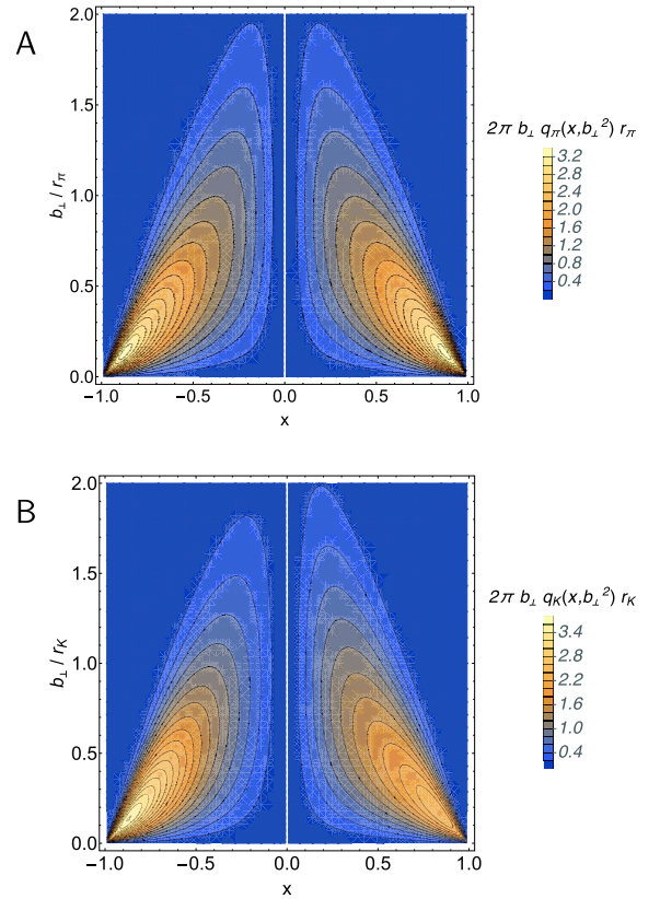
Fig. 10. (color online) Upper panel-A. Pion. IPS distributions for \bar{d} - (left) and u -quarks (right), charting the x -dependent probability density for locating these objects at distance |b_{\perp}| from the pion's centre of transverse momentum. Lower panel-B. Kaon. Analogous profiles for \bar{s} and u -quarks in the K^+ . Curves calculated using Eq. (31) and its analogues (based on factorised LFWF Ansätze , which yield the GPDs in Figs. 4, 5). In both panels, \zeta = \zeta_H .
