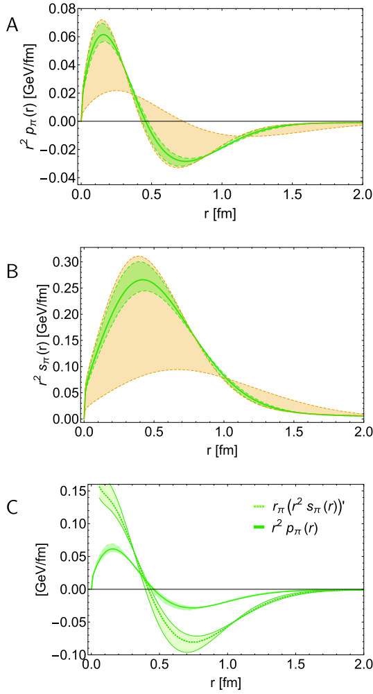
Fig. 14. (color online) Pion profiles. Upper panel-A : pressure. Middle panel-B : shear force. Green curve and band computed from obvious analogues of Eqs. (37), (45), with the terms in the second line of Eq. (37) evaluated using M = M_u(1 \pm 0.1) . Gold band: SCI results [30]. Lower panel-C : Pion pressure distribution in Panel A (solid green curve) compared with the derivative of the related shear force distribution in Panel B. (The r_\pi factor ensures matching units.) Both curves have near coincident zeros, revealing that shear forces are maximal in the neighbourhood of the radius whereat the pressure changes sign and confinement effects become dominant, Eq. (46).
