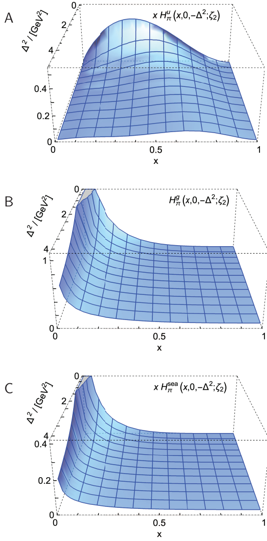
Fig. 17. (color online) Pion GPDs ( \xi = 0 ) computed in Sec. IV.B, beginning with the factorised LFWF and drawn in Fig. 4, evolved to \zeta_H \rightarrow \zeta_2 : Upper panel-A : valence; middle-B : glue; and lower-C : sea.
