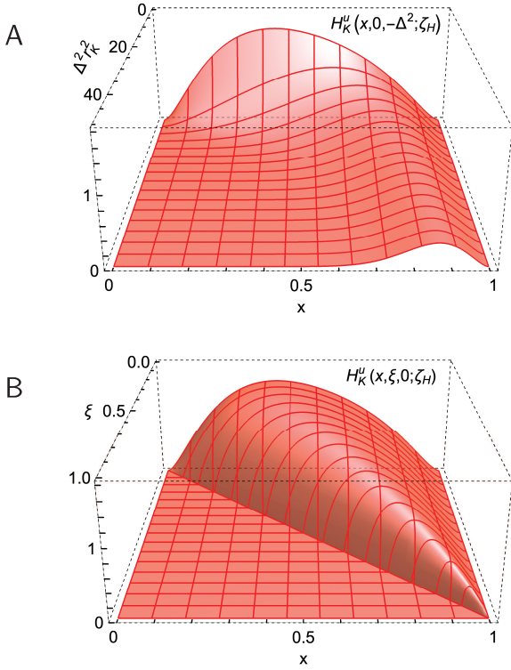
Fig. 5. (color online) Kaon GPD obtained using Eq. (11) and the factorised LFWF discussed in Sec. IV.B. Upper panel-A. H_K^u(x, \xi = 0, -\Delta^2; \zeta_H) . Lower panel-B. H_K^u(x, \xi, 0; \zeta_H) .
