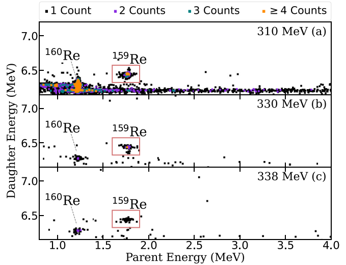
FIG. 5. Energy-energy correlation matrices for two consecutive decay events where the first decay occurred less than 10 s after an ion implantation in the same detector pixel and was followed within 12.5 ms by the second decay. No more than two signals were observed in JYTube in association with the evaporation residue. The spectra were measured at beam energies of (a) 310 MeV, (b) 330 MeV, and (c) 338 MeV. Groups identified as proton decays of ^{159}\text{Re} and ^{160}\text{Re} correlated with their daughter \alpha decays are labeled.
