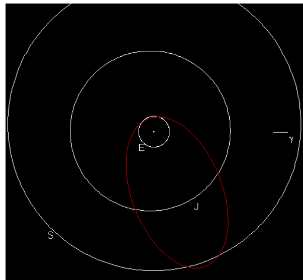
Figure 2. Heliocentric orbit of the SPMN270411 sporadic fireball. For comparison, the orbits of Saturn, Jupiter and Earth are also shown.
