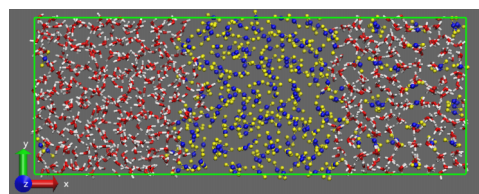
FIG. 2. Snapshot of the initial configuration formed by a slab of liquid CO 2 surrounded by a slab of CO 2 hydrate and a slab of liquid H 2 O molecules. H 2 O molecules are plotted in red and white and CO 2 molecules in blue and yellow. The initial box dimensions are x = 72 \text{ \AA} , y = 24 \text{ \AA} , and z = 24 \text{ \AA} .
