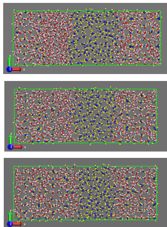
FIG. 6. Snapshots of layer by layer CO 2 hydrate growth, beginning at the interface of liquid H 2 O-initial hydrate slab and eventually reaching the hydrate-liquid CO 2 equilibrium.
