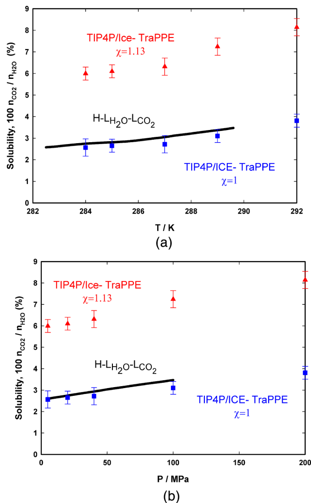
FIG. 11. (a) T-x and (b) P-x projections of the estimated CO 2 solubility values in H 2 O, along the three phase line. Solid line represents the experimental correlation by Diamond and Akinfiev, 84 and the symbols are MS results using TIP4P-Ice H 2 O and TraPPE CO 2 , using Lorentz Berthelot rules with \chi = 1 (blue squares) and \chi = 1.13 (red triangles).
