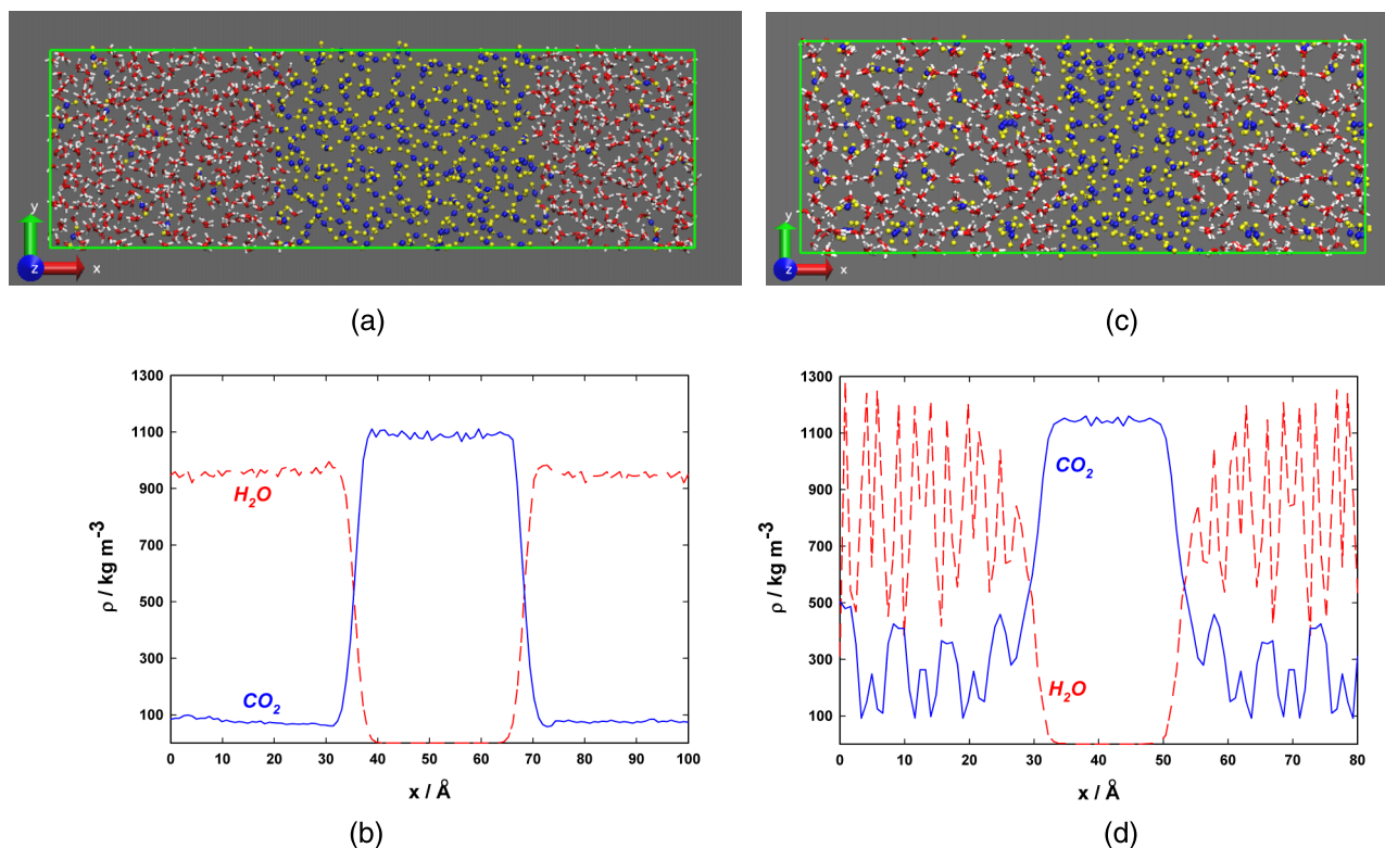
FIG. 5. Snapshots of the final states with their corresponding density profiles along the x -axis at 100 MPa. (a) and (b) Liquid H 2 O (TIP4P-Ice) and liquid CO 2 (TraPPE) at 275 K; (c) and (d) hydrate and liquid CO 2 at 270 K. H 2 O molecules are plotted in red and white and CO 2 molecules in blue and yellow.
