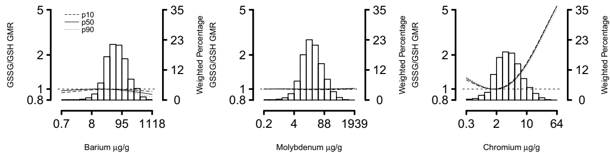
Fig. 1. GMR of GSSG/GSH by Ba, Mo and Cr concentrations when the other two metals are fixed at their 10th, 50th and 90th percentiles.
