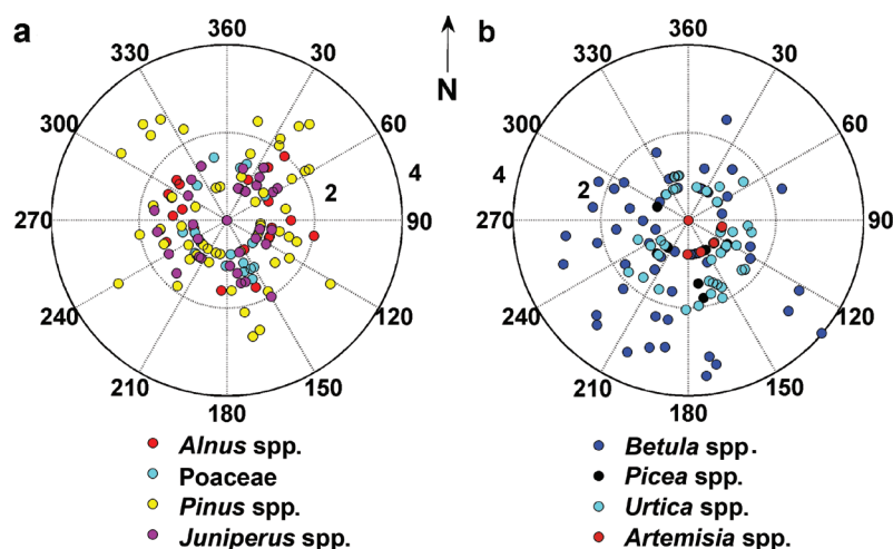
Fig. 3. Pollen concentration [log(grains per m 3 )] as a function of local wind direction in 2003. (a) Species whose pollen concentrations are independent of local wind direction, and (b) species, whose pollen originates mostly from wind directions 120°–270°.
