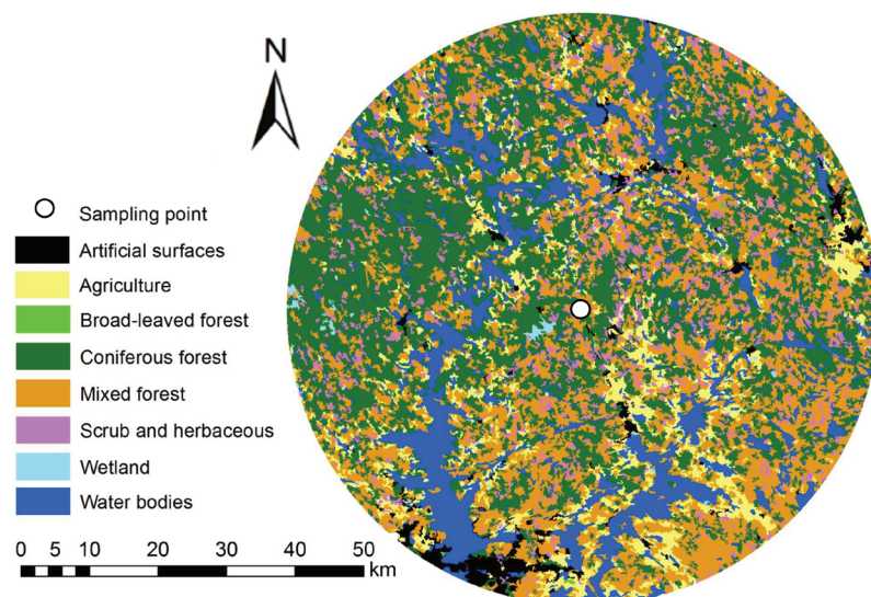
Fig. 1. Land-use map extracted from the Corine database for 50 km radius around the Hyytiälä forest site (EEA 1997, Williams et al. 2011).
