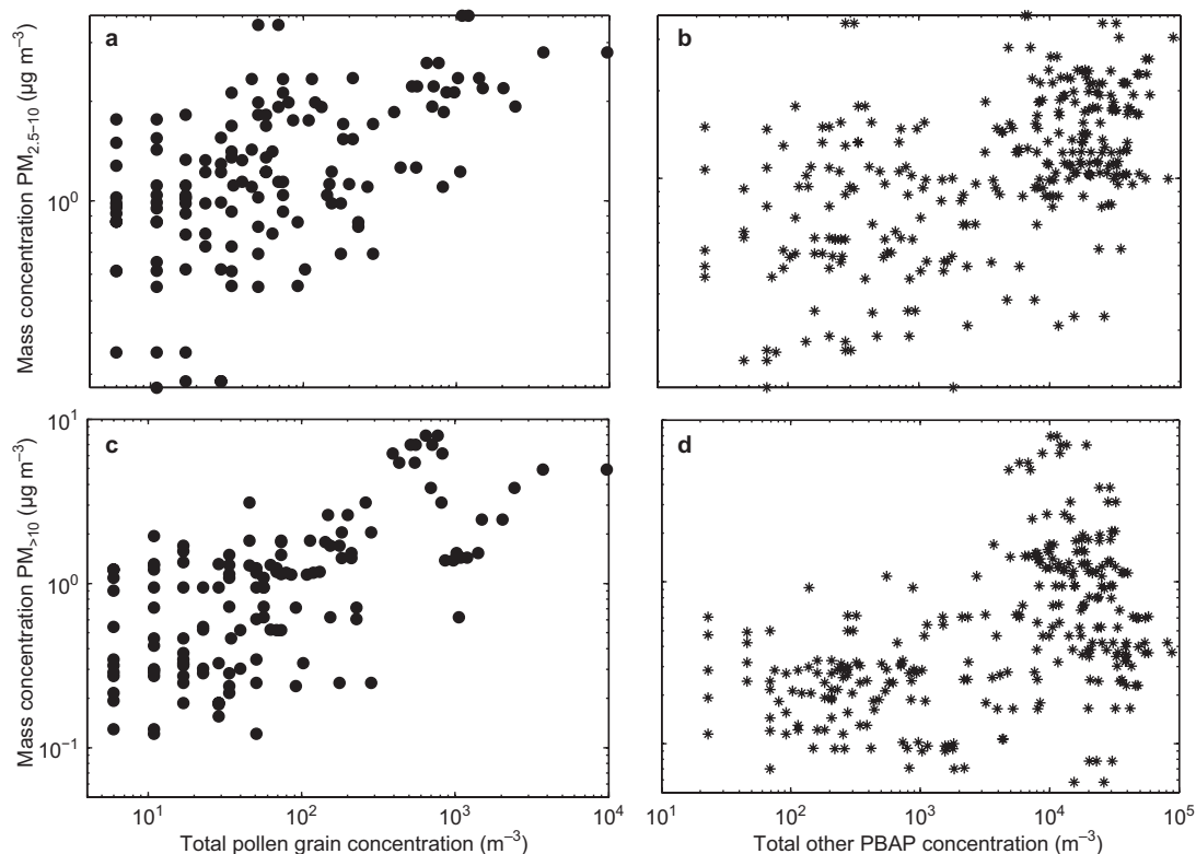
Fig. 7. Relationships between 2–3 day average particle mass concentrations of PM_{2.5-10} (a, b) and PM_{>10} (c, d), and total pollen (a, c) or other PBAP number concentrations (b, d) during the PBAP season in Hyttiälä.
