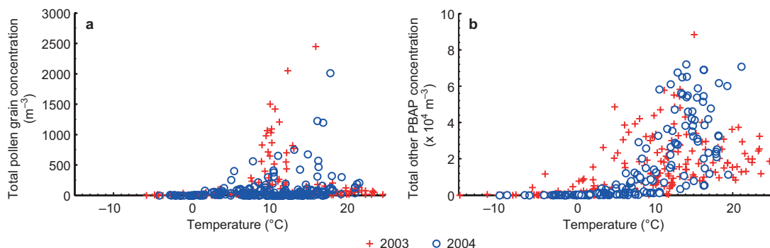
Fig. 8. Relations between (a) total pollen grain concentration and (b) other PBAP concentration, and daily mean temperature in 2003–2004 in Hyytiälä during the PBAP season.
