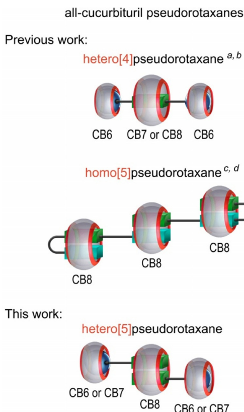
Scheme 1. Examples of all-CB pseudorotaxanes and representation of the target structures in this study. [a] Ref. [39]. [b] Ref. [40]. [c] Ref. [36]. [d] Ref. [46].
