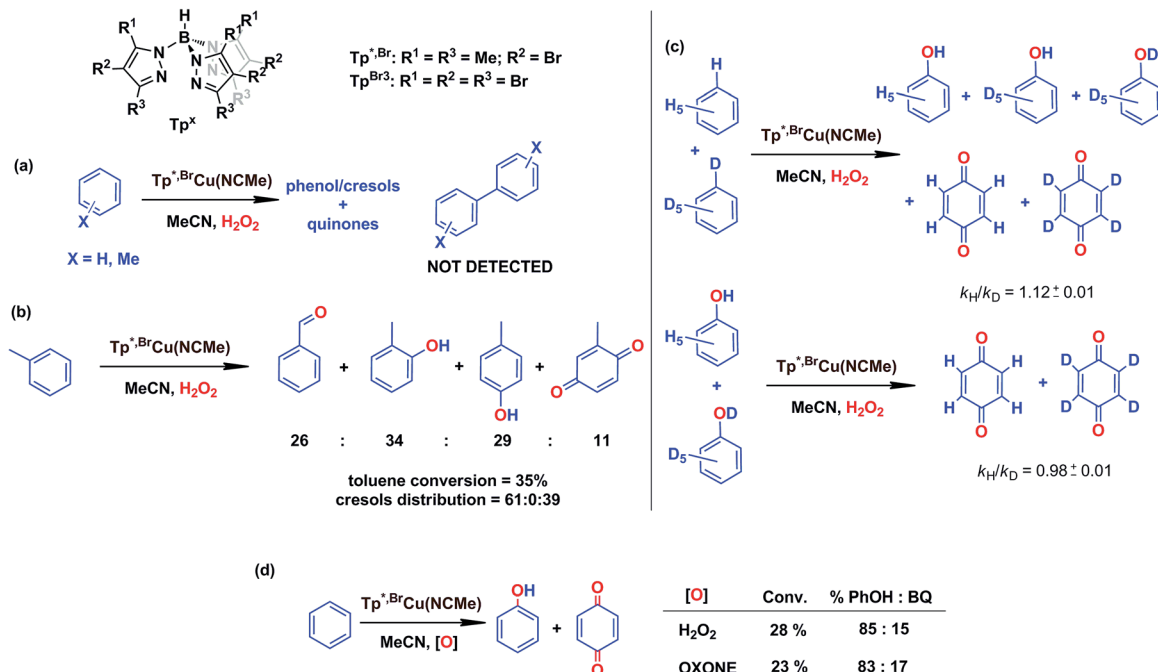
Scheme 4 Evidences collected to discard the existence of a Fenton-like mechanism in the Tp^*Cu(NCMe) -catalysed hydroxylation of benzene. Reaction conditions: 0.01 mmol catalyst in 2–3 mL of acetonitrile (see ESI† for details in each case) and 5–10 mmol of the arene (or mixture of protio and deuterio benzenes). Reaction time: 5–8 h at 80 °C. H_2O_2 is employed in excess compared to the arene.
