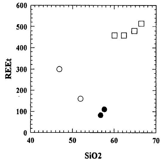
Fig. 2.- A) Chondrite normalized REE patterns for the Toledo gabbros, Argés quartz-diorites - tonalites and Argés granodiorites and granites. B) Total REE vs. SiO 2 variation diagram. Symbols as in figure 1.
