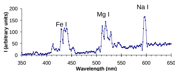
Figure 2. Spectrum corresponding to the final flare of a Kappa Cygnid fireball registered on August 23, 2007.
