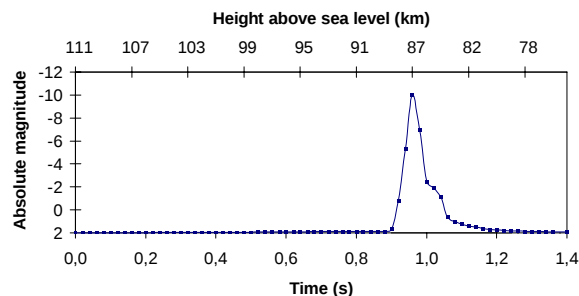
Figure 1. Photometric curve of a Kappa Cygnid fireball registered on August 23, 2007.
