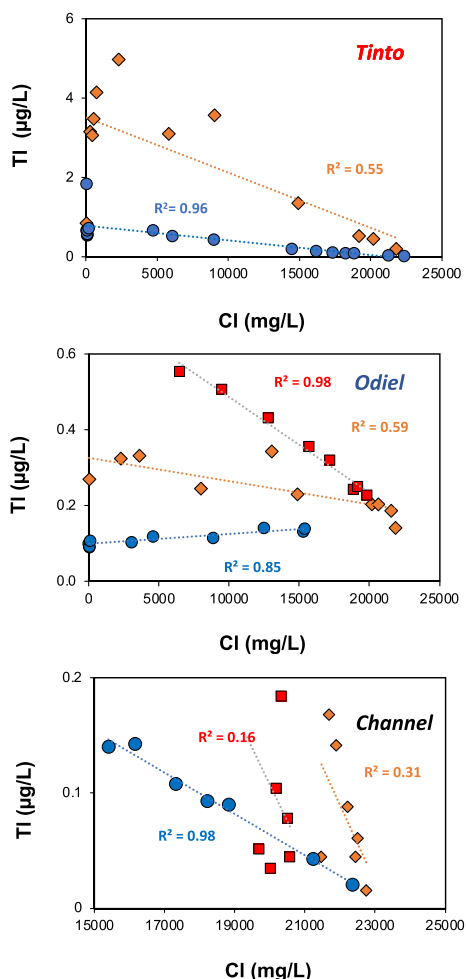
Fig. 2. Relationship between dissolved Tl and Cl concentrations in the different estuarine domains of the Ría de Huelva. Dry season: orange diamonds; Wet season: blue circles; and Odiel Mine spill: red squares. (For interpretation of the references to colour in this figure legend, the reader is referred to the Web version of this article.)
