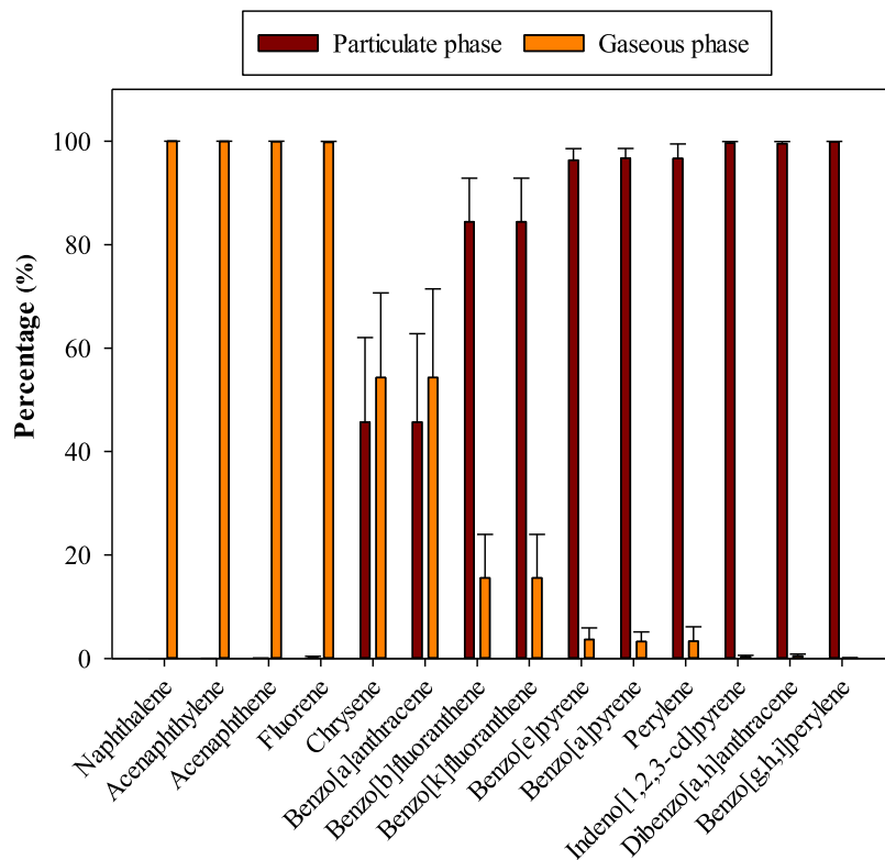
Fig. 5 – Partition of PAHs between the gas and particle phases.
