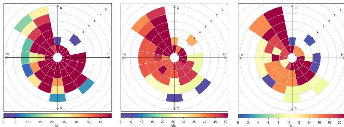
Fig. 2 – Pollution roses for the most abundant metals. Wind speeds and concentrations are given in m/sec and ng/m 3 , respectively.
